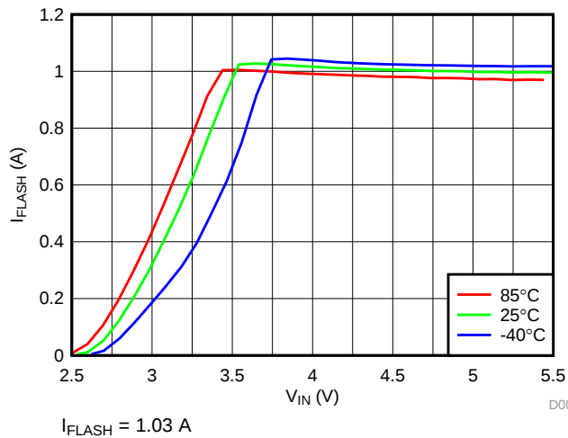
图 4. LED Flash Current vs Input Voltage
