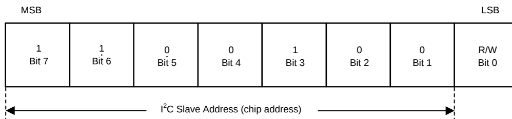
FIG 23. I 2 C-Compatible Chip Address
