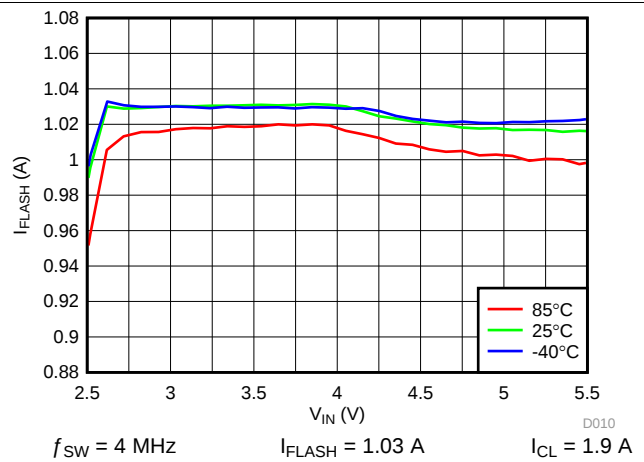
FIG 11. LED Flash Current vs Input Voltage
