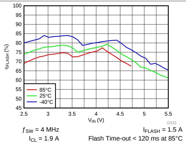
FIG 43. LED Flash Efficiency vs Input Voltage
