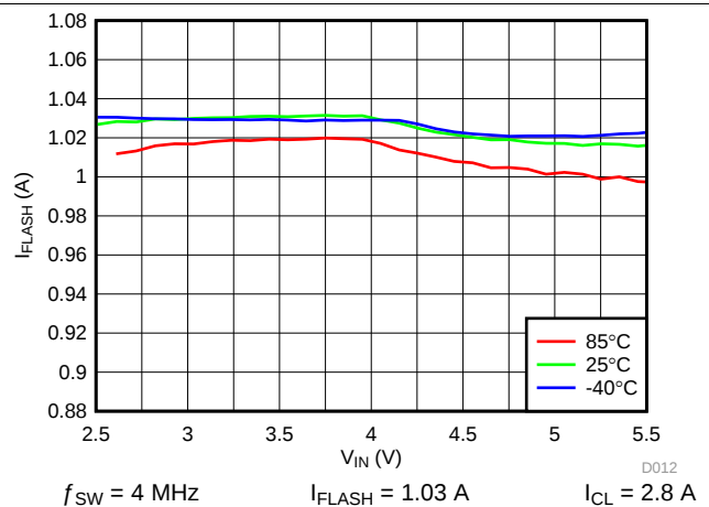
FIG 13. LED Flash Current vs Input Voltage
