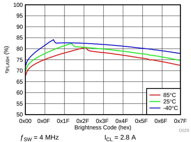
FIG 39. LED Flash Efficiency vs Brightness Code
