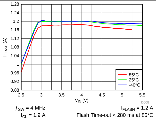
FIG 9. LED Flash Current vs Input Voltage
