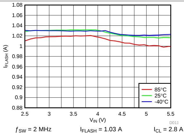
FIG 12. LED Flash Current vs Input Voltage
