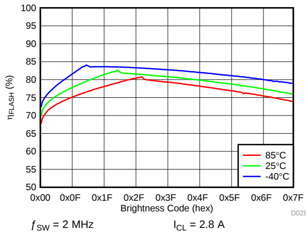
FIG 38. LED Flash Efficiency vs Brightness Code
