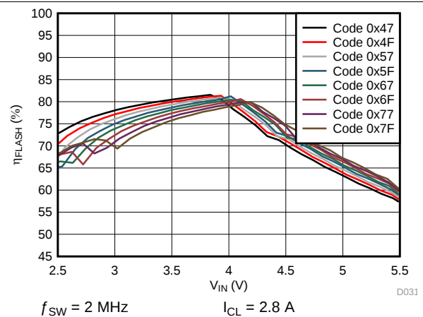
FIG 41. LED Flash Efficiency vs Input Voltage
