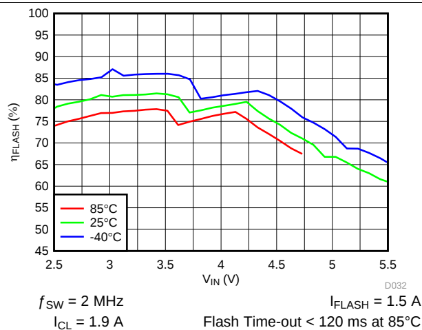
FIG 42. LED Flash Efficiency vs Input Voltage
