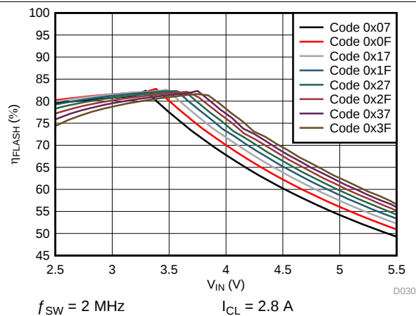
FIG 40. LED Flash Efficiency vs Input Voltage
