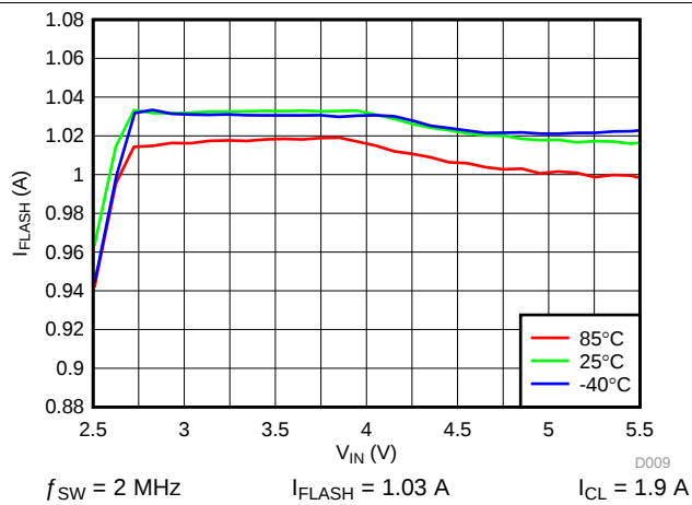
FIG 10. LED Flash Current vs Input Voltage
