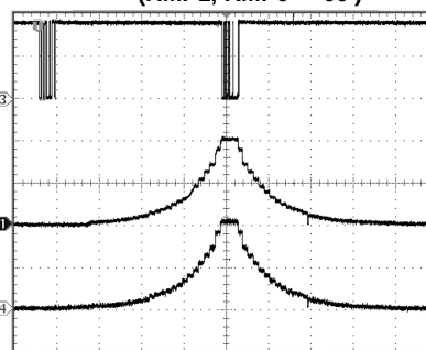
Ramp Rate Functionality (RMP1, RMP0 = '00')
