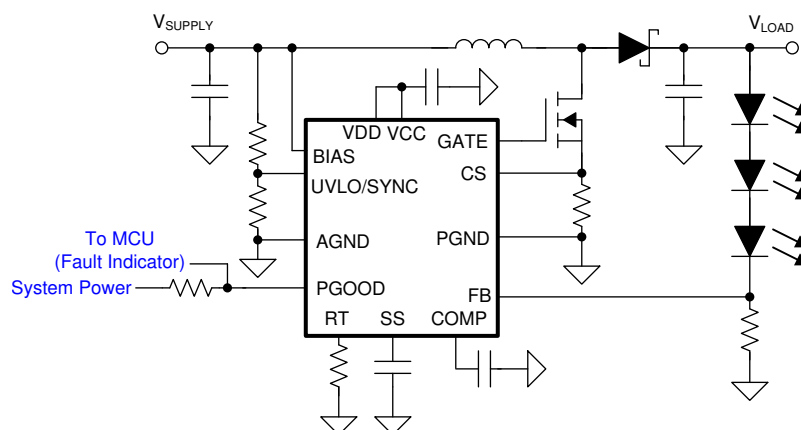
9-9. Low-Cost LED Driver
