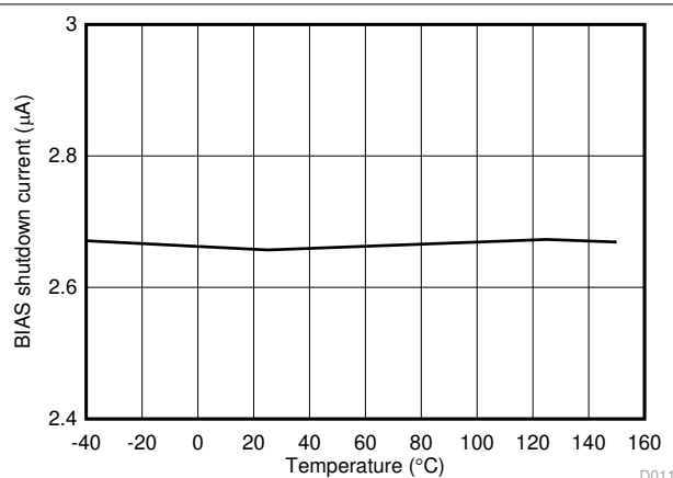
7-11. I_{\text{SHUTDOWN}} vs Temperature (BIAS = 12 V)
