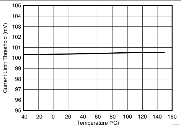
7-6. Current Limit Threshold vs Temperature
