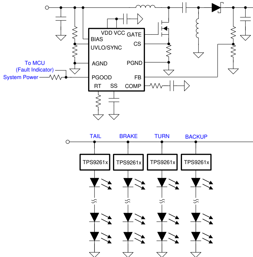
9-14. Dual-Stage Automotive Rear-Lights LED Driver
