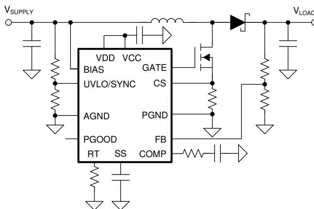
FIG 9-3. Typical Boost Application
