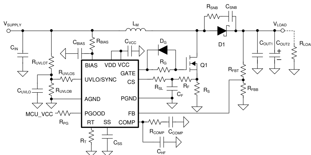
9-1. Typical Boost Converter Circuit With Optional Components
