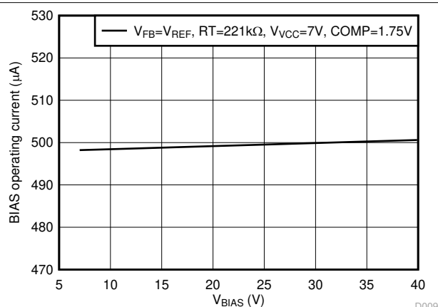
7-9. I_{\text{OPERATING(BIAS)}} Including RT Current vs V_{\text{BIAS}}
