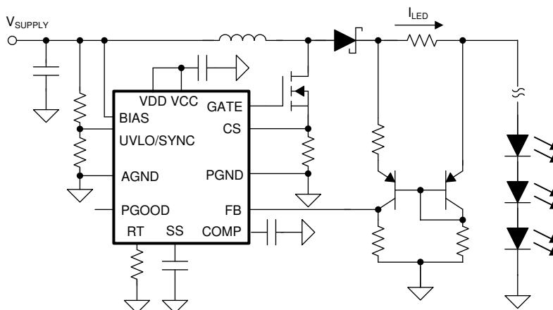
9-13. LED Driver with High-Side Current Sensing
