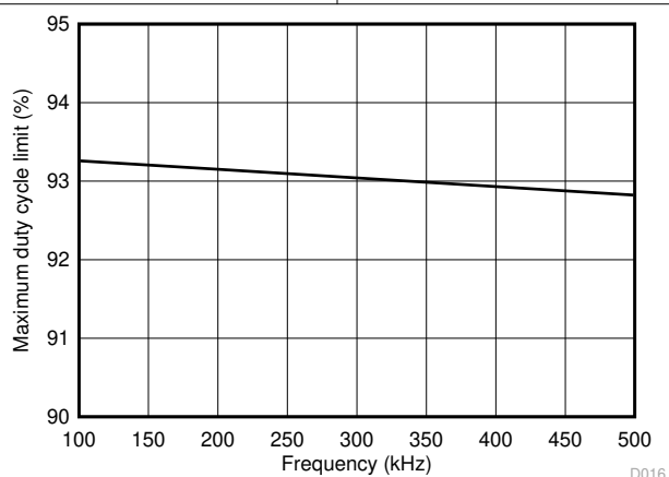
7-15. Maximum Duty Cycle vs Frequency
