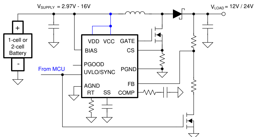
9-4. Typical Start-Stop Application
