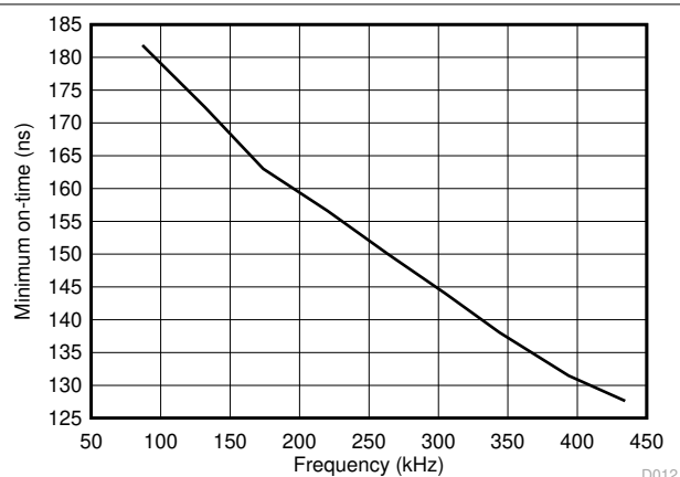
7-12. t_{\text{ON(MIN)}} vs Frequency
