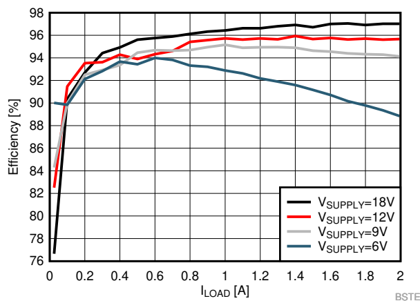
FIG 9-2. Efficiency
