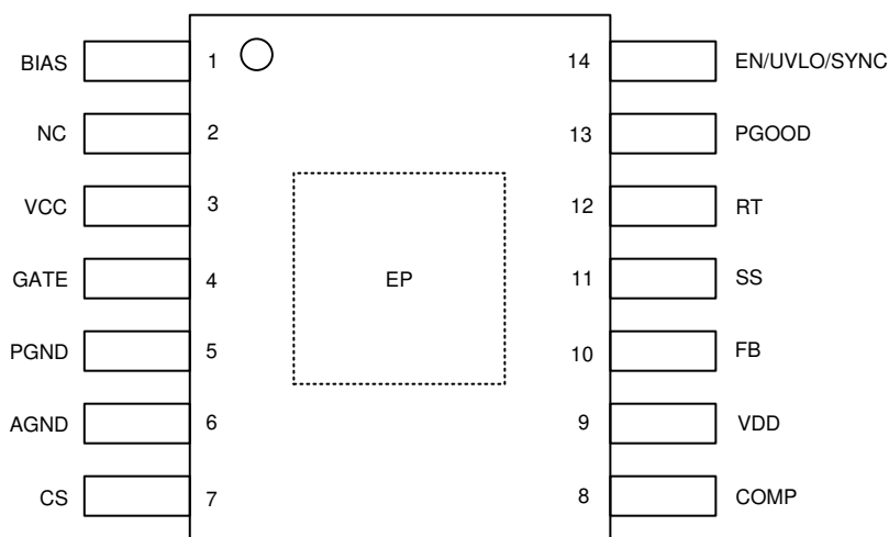
FIG 6-1. 14-Pin HTSSOP PWP Package (Transparent Top View)
