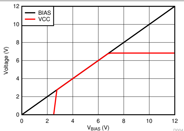
7-4. V VCC vs V BIAS (No Load)
