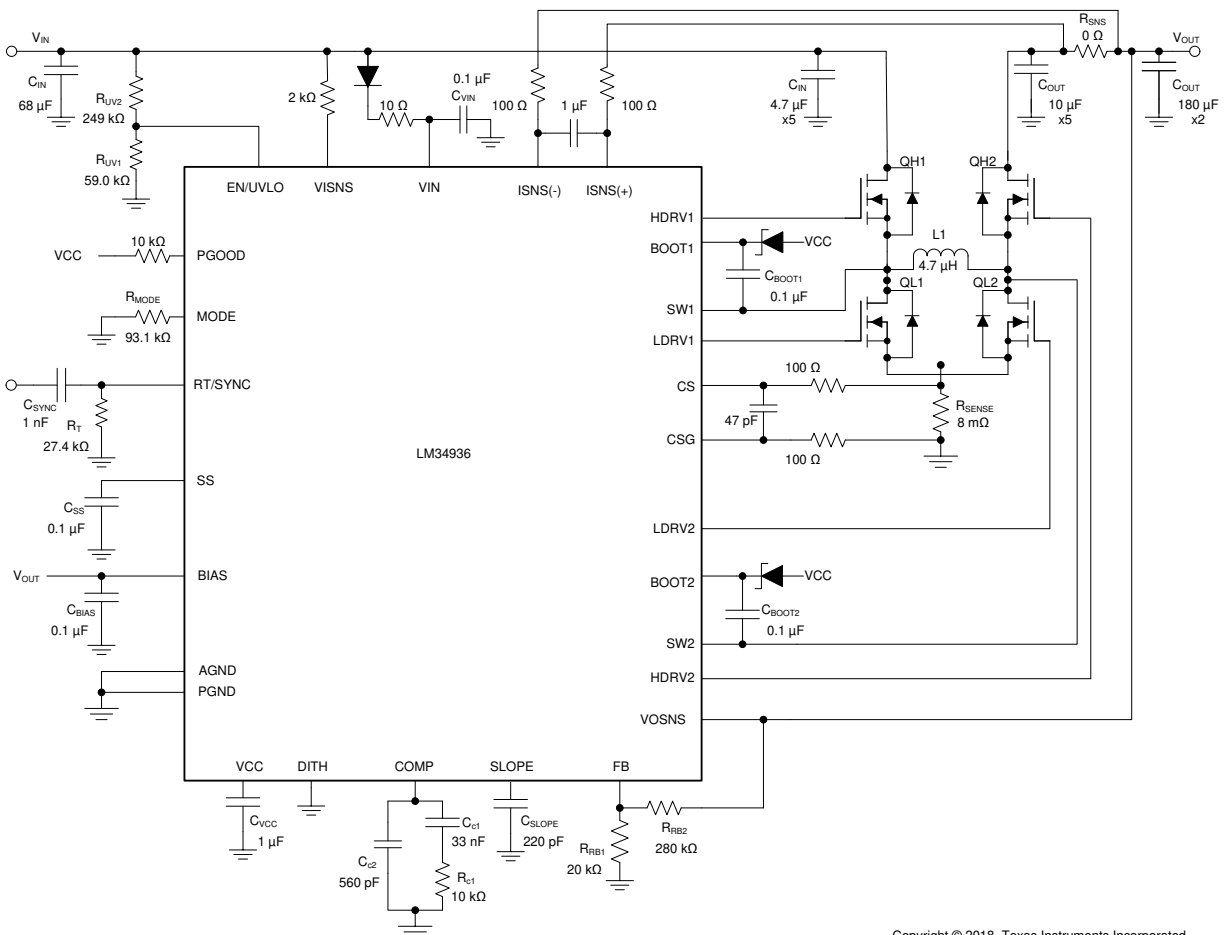
8-1. LM34936 Four-Switch Buck Boost Application Schematic
