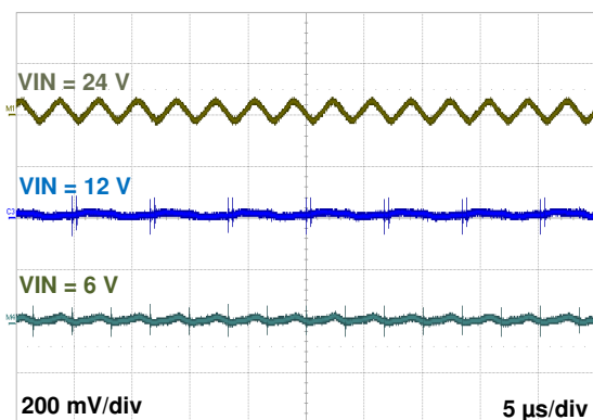
8-4. Output Voltage Ripple
