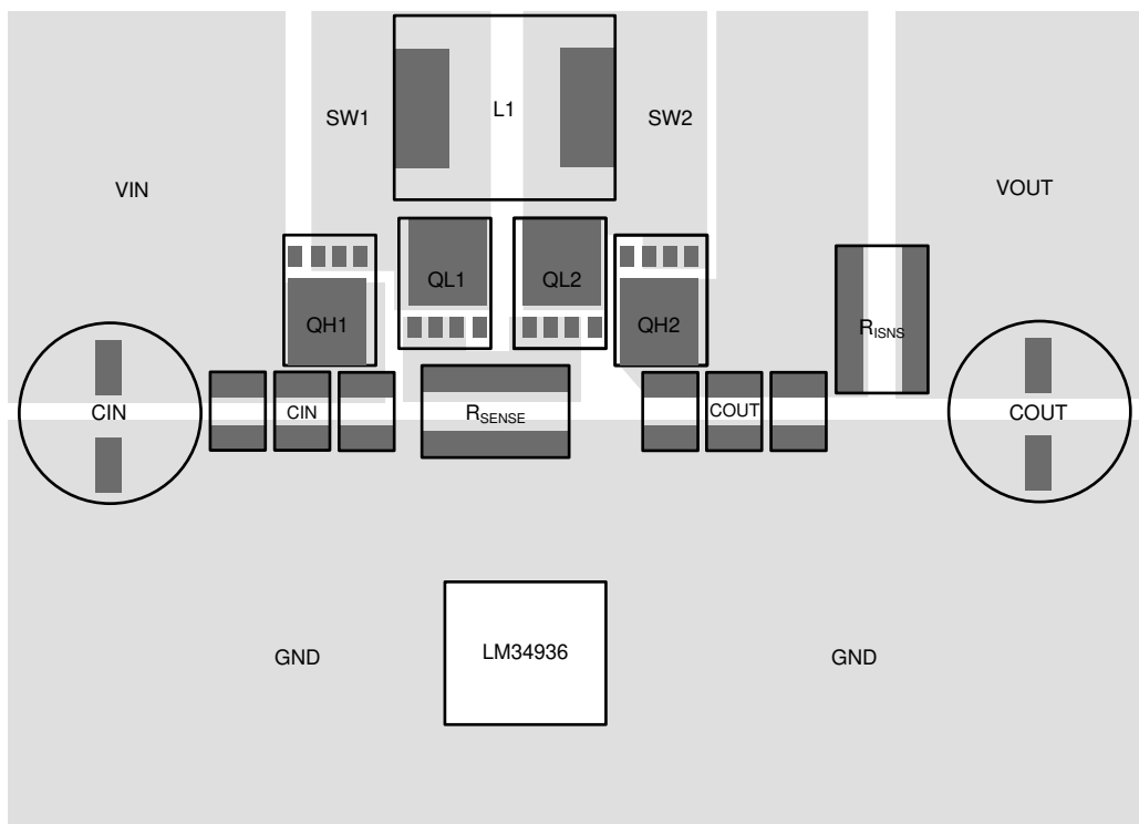
10-1. LM34936 Power Stage Layout
