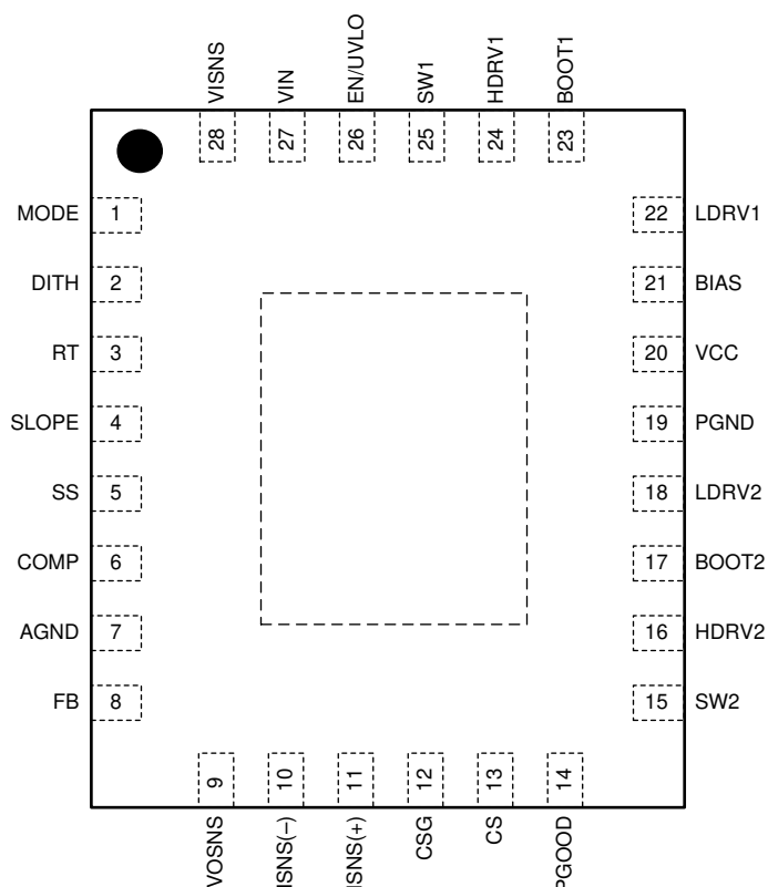
5-1. QFN-28 RHF Package Top View
