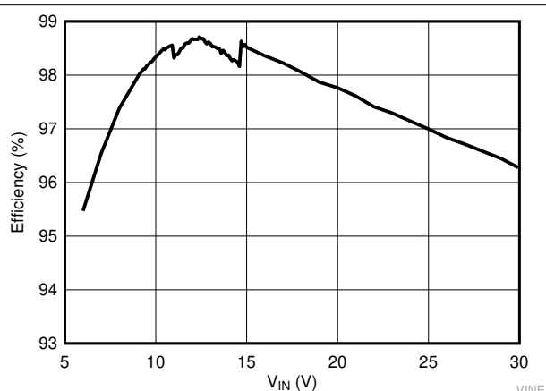
8-3. Efficiency vs Input Voltage
