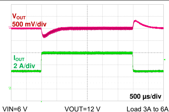
6-15. Load Step (Boost)
