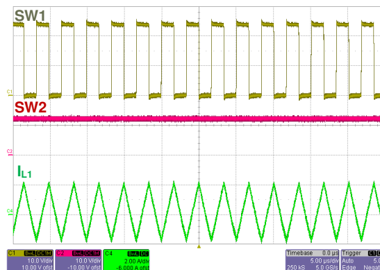
6-14. Forced CCM Operation (Buck)
