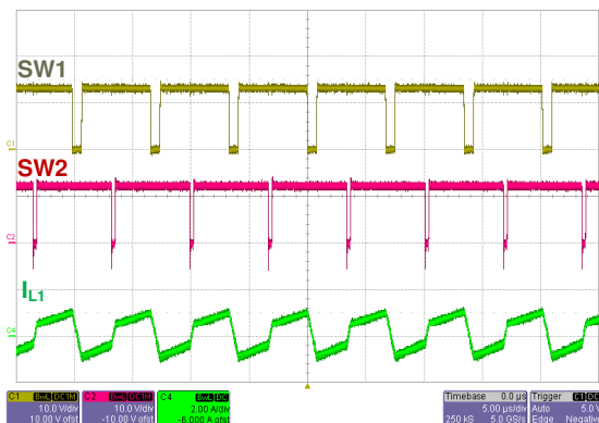
6-13. Forced CCM Operation (Buck-Boost)
