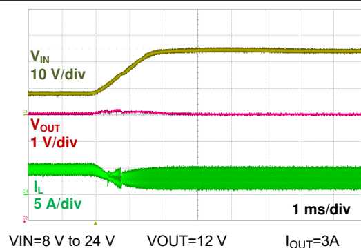
6-18. Line Transient
