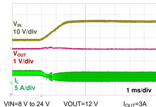
Figure 6-18. Line Transient
