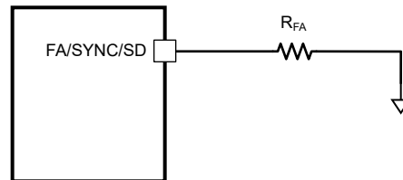
図 6-8. Frequency Adjust
