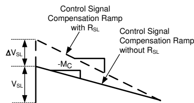
図 6-5. Additional Slope Compensation Added Using External Resistor R_{SL}
