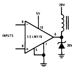
Figure 25. Relay Driver
