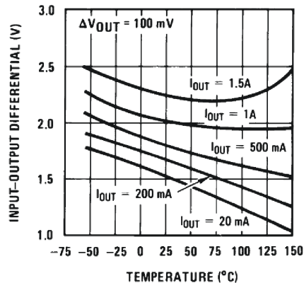
図 6-18. Dropout Voltage vs Temperature (New Chip)
