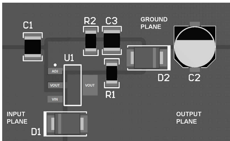
図 8-24. SOT-223 Layout Example (New Chip)
