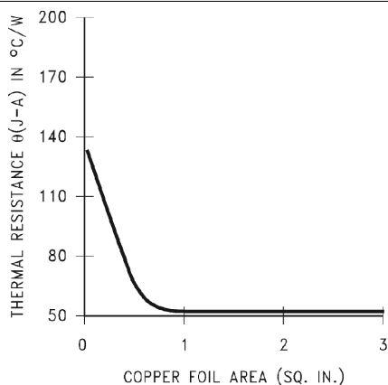
図 8-19. R_{\theta JA} vs Copper (2oz.) Area for the SOT-223 Package
