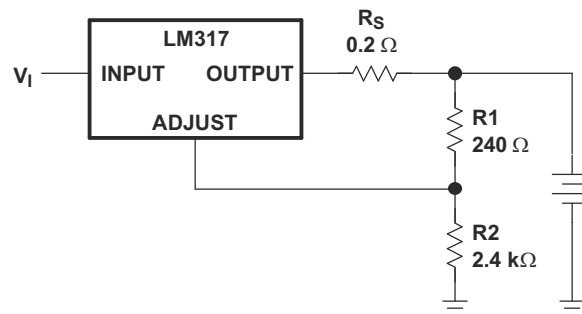
図 8-11. Battery-Charger Circuit
