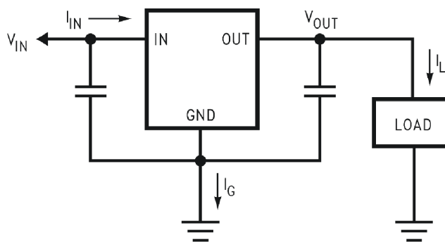
図 8-18. Power Dissipation Diagram
