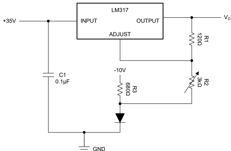
図 8-6. 0V to 30V Regulator Circuit
