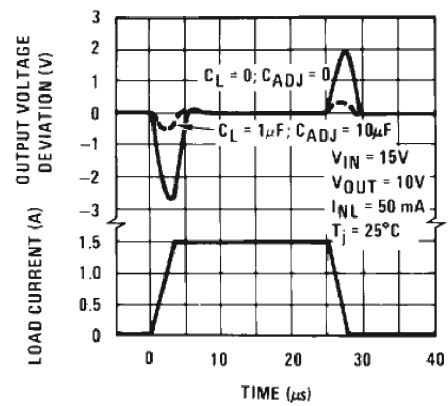
図 6-4. Load Transient Response (Legacy Chip)
