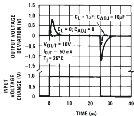
図 8-2. Line-Transient Response (Legacy Chip)
