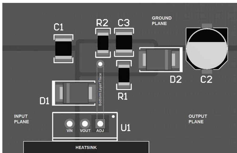
図 8-25. TO-220 Layout Example (New Chip)
