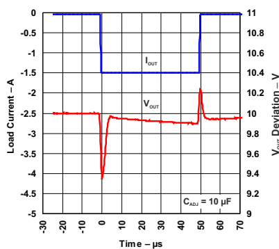
図 6-3. Load Regulation (New Chip)
