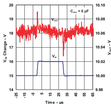
図 8-2. Line-Transient Response (Legacy Chip)
