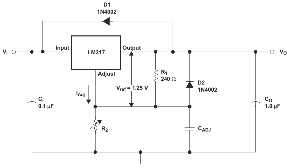
図 8-1. Adjustable Voltage Regulator
