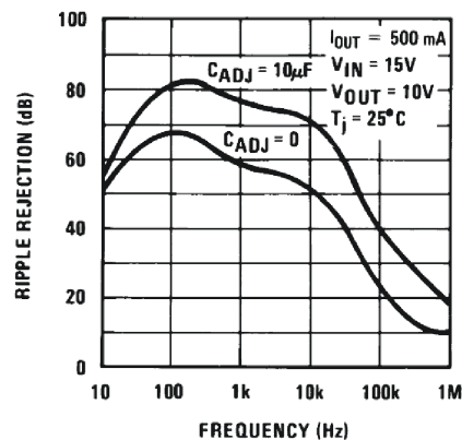
図 6-14. Ripple Rejection vs Frequency (New Chip)
