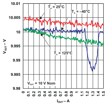
図 6-1. Load Regulation (Legacy Chip)
