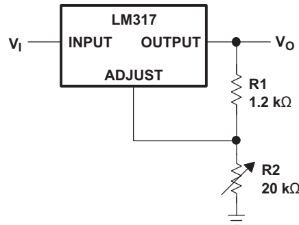
図 8-10. 1.25V to 20V Regulator Circuit With Minimum Program Current
