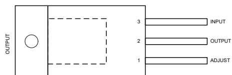
図 5-2. KCS or KCT Package, 3-Pin TO-220 (Top View), Legacy Chip
