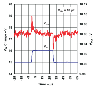
図 8-3. Line-Transient Response (Legacy Chip)
