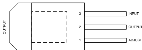
図 5-3. KTT Package, 3-Pin TO-263 (Top View)
