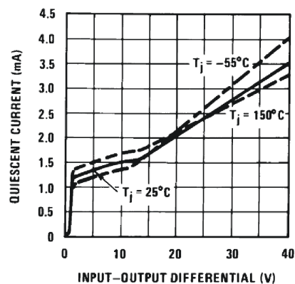
図 6-20. Minimum Operating Current (New Chip)
