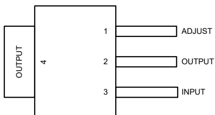
図 5-1. DCY Package, 4-Pin SOT-223 (Top View)
