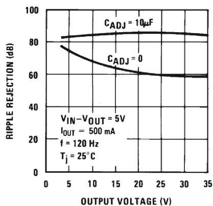
図 6-13. Ripple Rejection vs Output Voltage (New Chip)
