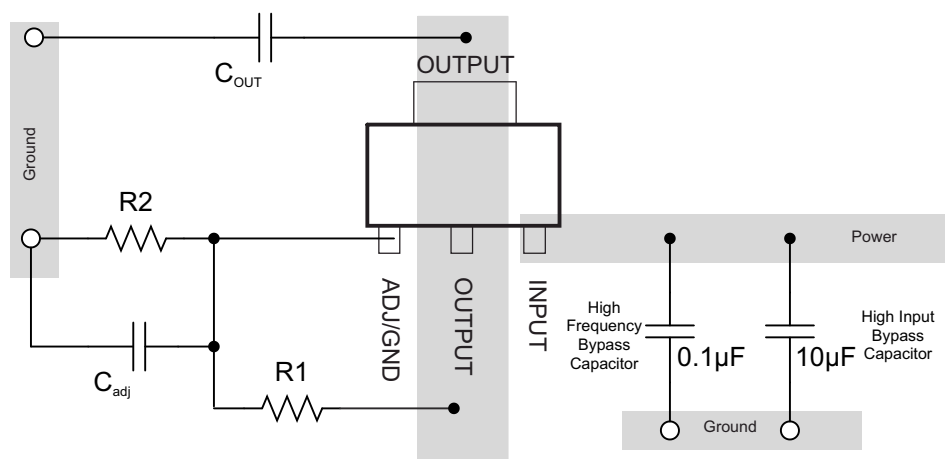
図 8-23. Layout Example (Legacy Chip)
