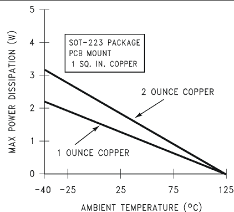
図 8-20. Maximum Power Dissipation vs T_{AMB} for the SOT-223 Package
