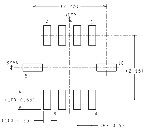
RECOMMENDED LAND-PATTERN
