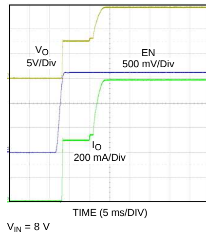
Figure 12. Start-Up Waveforms
