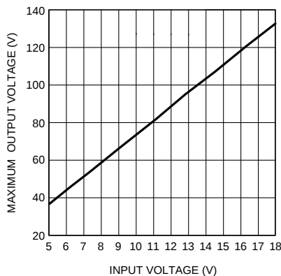
Figure 18. Maximum Output Voltage
