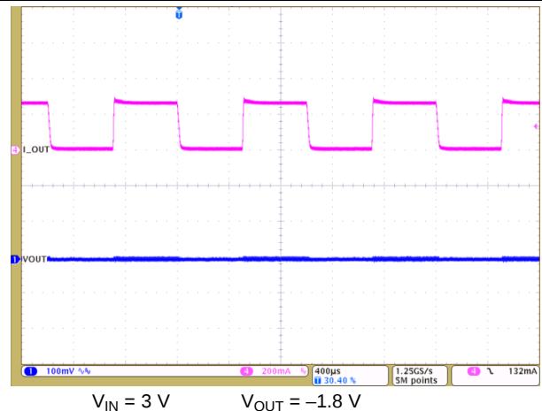
Figure 21. Load Step
