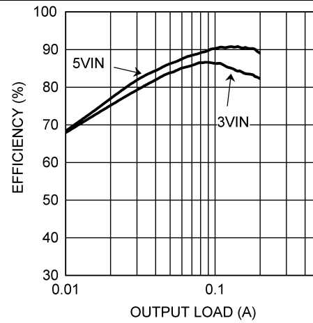
Figure 8. LM2735Y Efficiency vs Load Current
