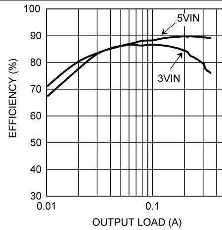
Figure 10. LM2735Y Efficiency vs Load Current
