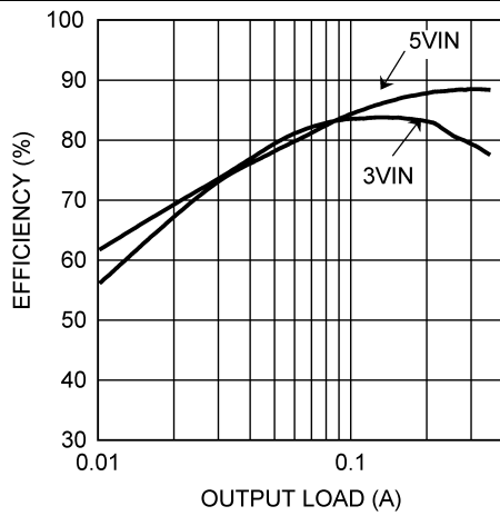
Figure 9. LM2735X Efficiency vs Load Current
