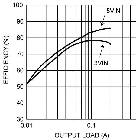
Figure 7. LM2735X Efficiency vs Load Current
