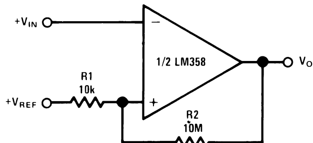
8-15. Comparator with Hysteresis
