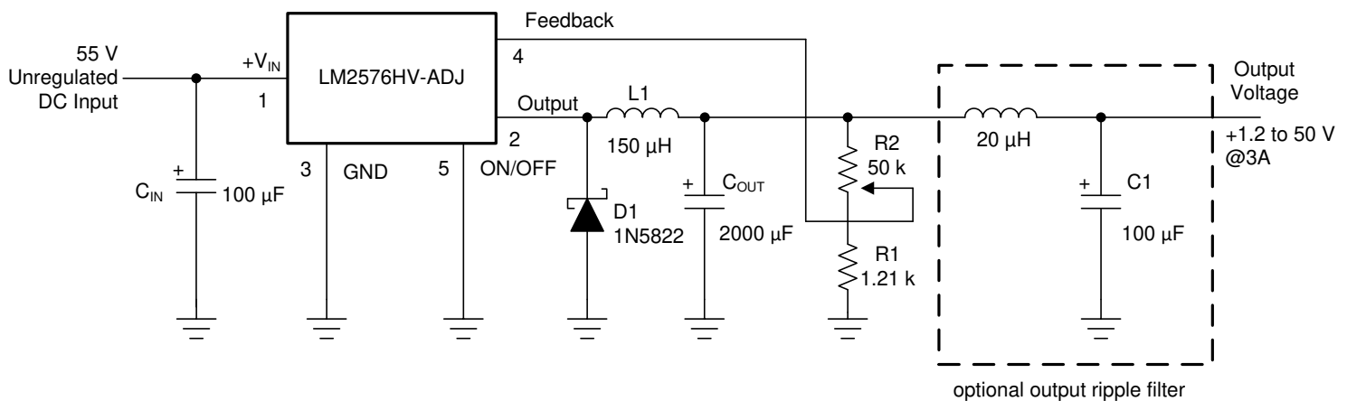
図 7-4. 1.2-V to 55-V Adjustable 3-A Power Supply With Low Output Ripple
