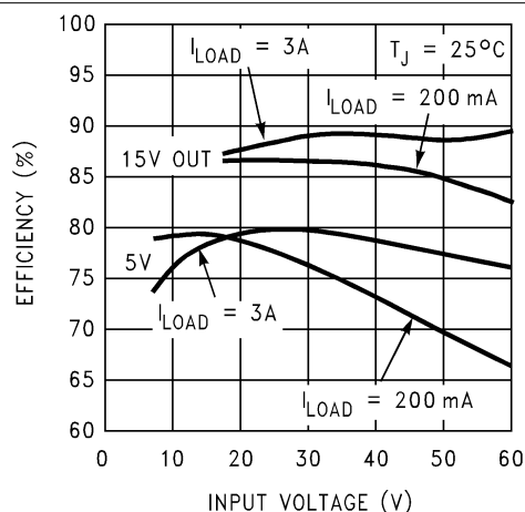
6-9. Efficiency
