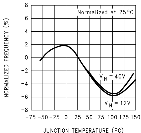
6-7. Oscillator Frequency
