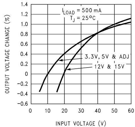
Figure 6-2. Line Regulation
