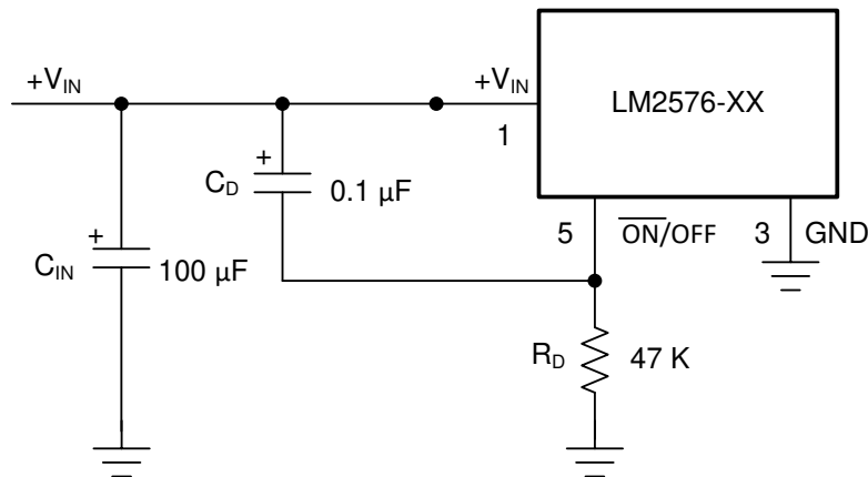
図 7-3. Delayed Start-Up
