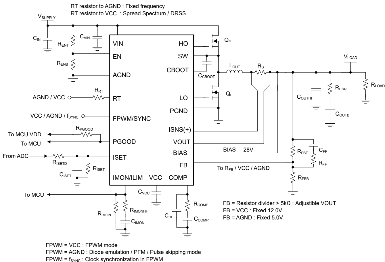
7-4. Typical CC-CV Buck Regulator Circuit
