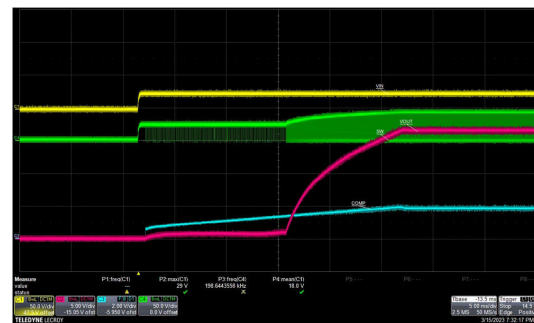
V_{IN} stepped to 24 V 1-A Load
