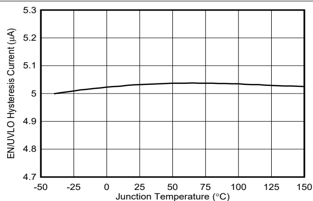
図 6-9. EN/UVLO Hysteresis Current versus Temperature
