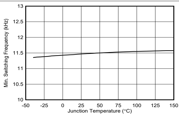
図 6-12. Minimum Switching Frequency versus Temperature
