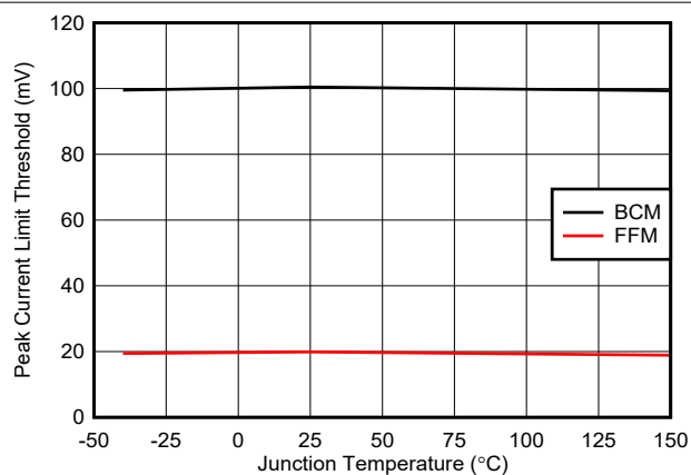
図 6-10. Peak Current Limit Thresholds vs. Temperature
