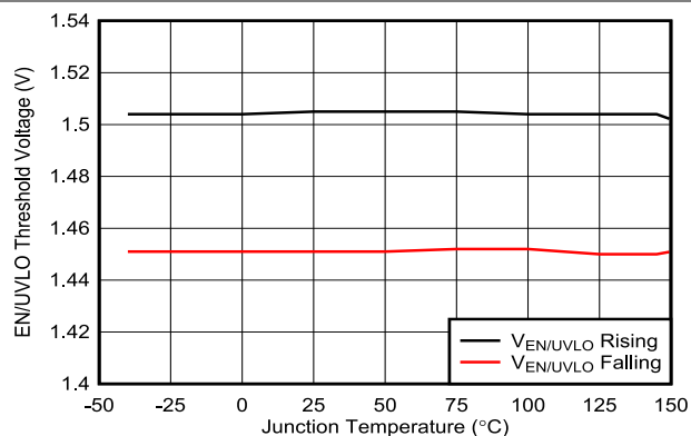
図 6-8. EN/UVLO Threshold Voltages versus Temperature
