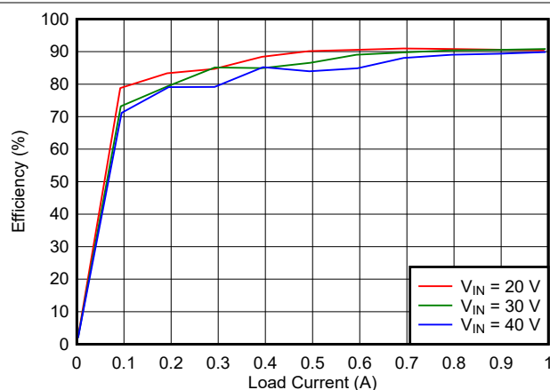
図 6-1. Efficiency versus Load
