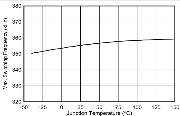
図 6-13. Maximum Switching Frequency versus Temperature
