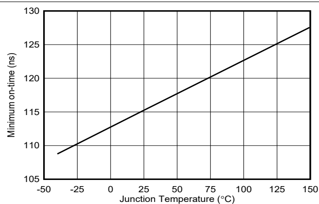
図 6-11. Minimum Switch On-Time versus Temperature
