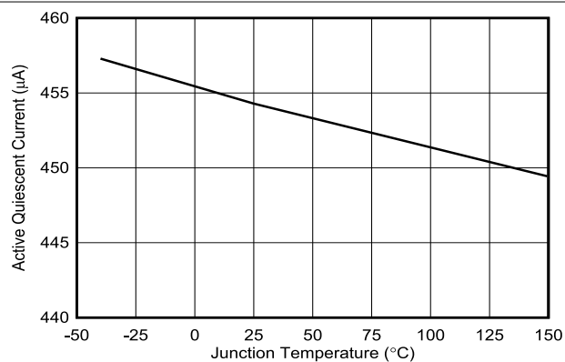
図 6-4. Active Quiescent Current vs. Temperature
