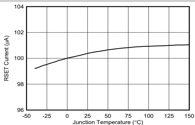
図 6-6. RSET Current versus Temperature
