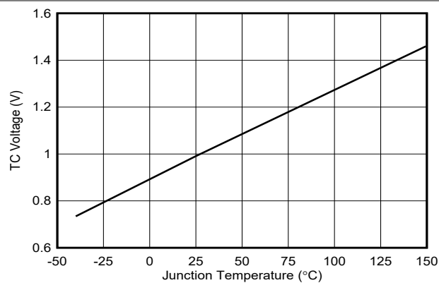
図 6-7. TC Voltage versus Temperature
