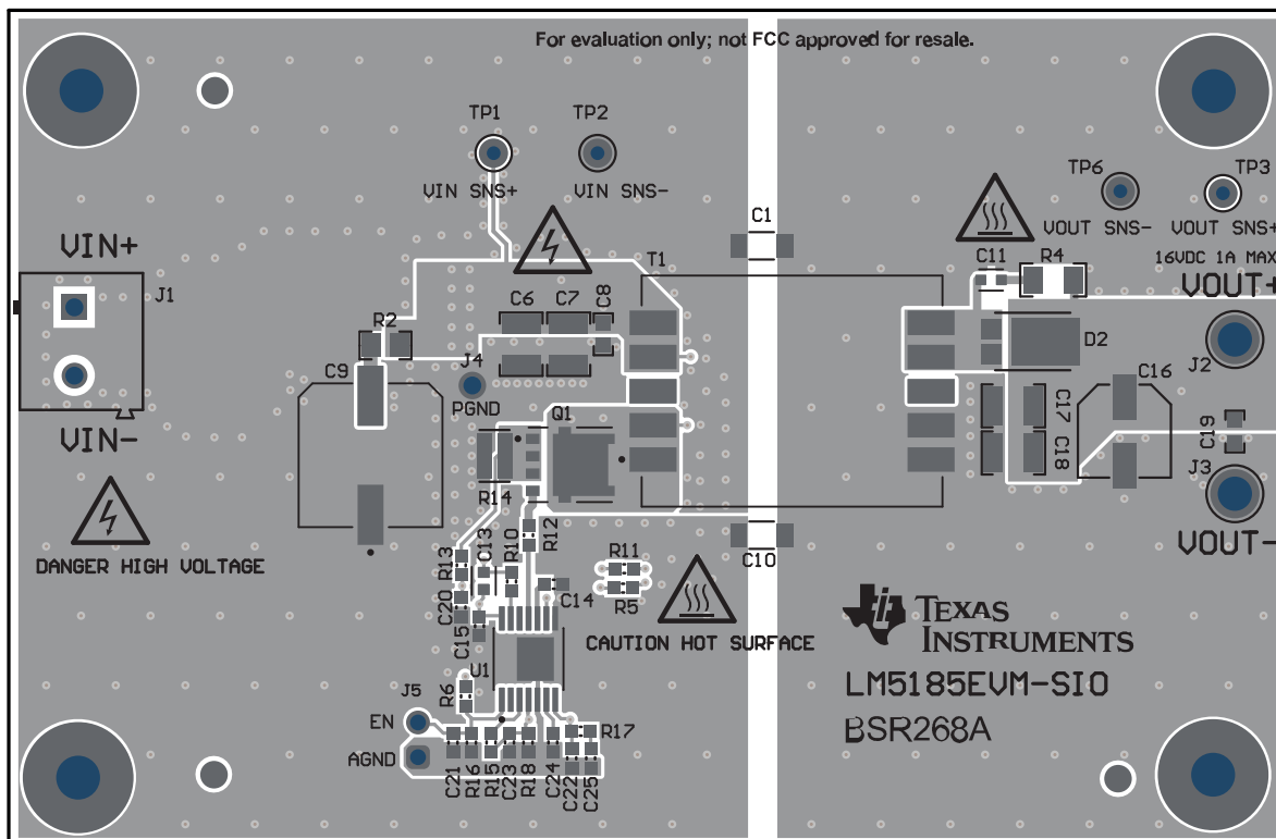
図 8-6. Single-Output PCB Layout Example
