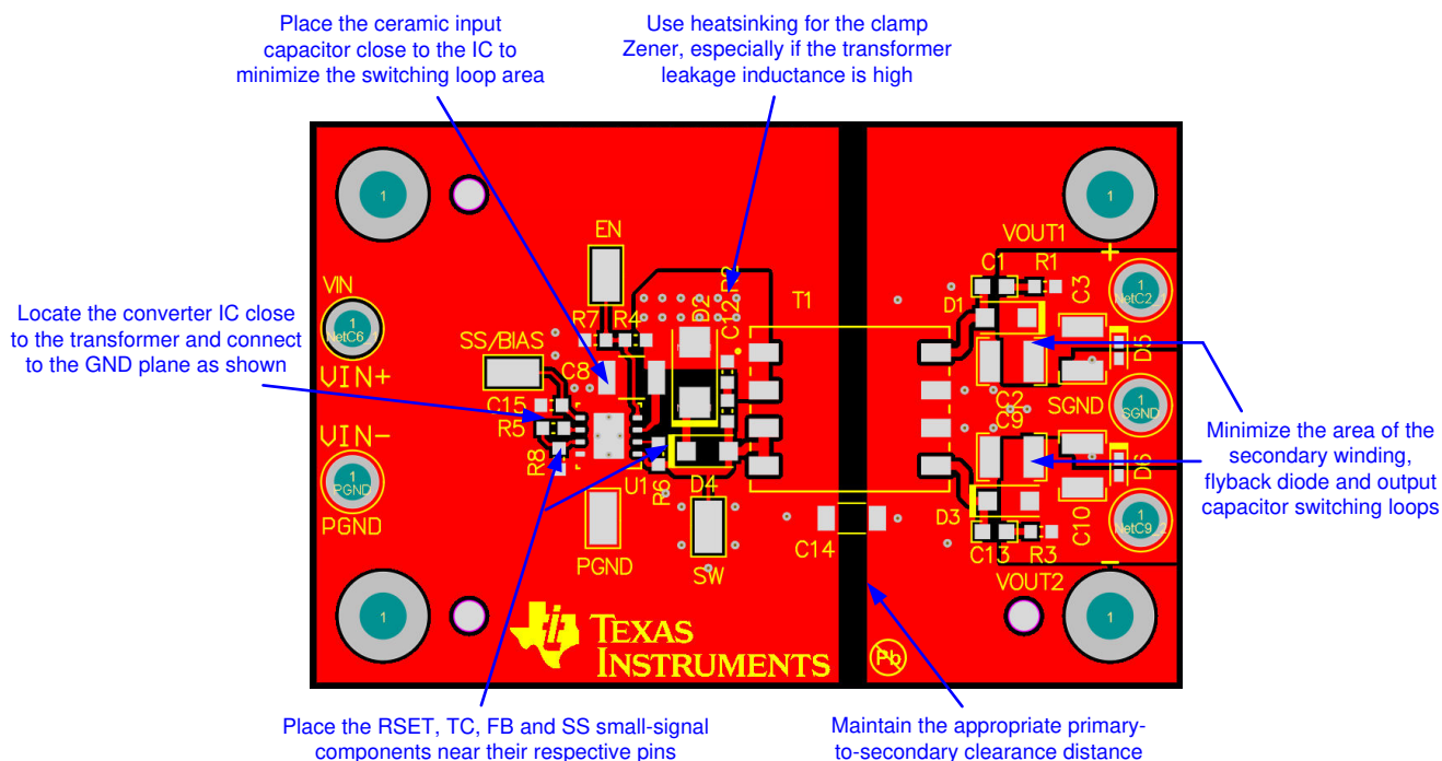
FIG 10-2. Dual-Output PCB Layout Example
