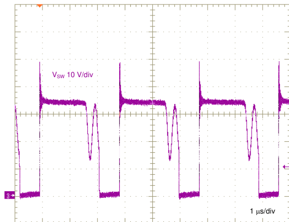
V_{IN} = 24\text{ V} I_{OUT1} = I_{OUT2} = 0.3\text{ A} 図 8-23. Switch Voltage, Medium Load
