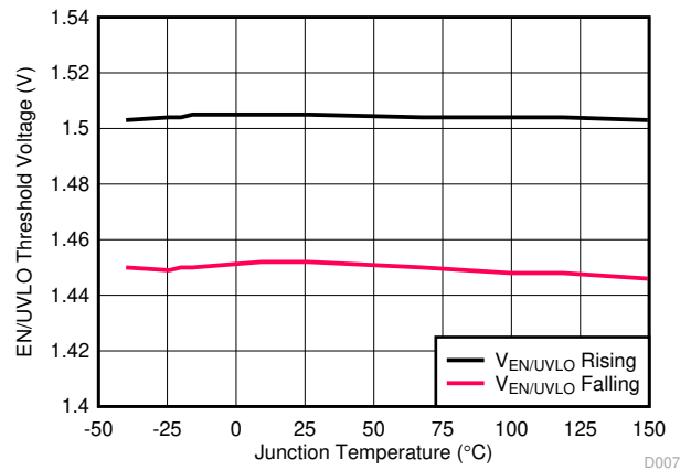
FIG 6-10. EN/UVLO Threshold Voltages versus Temperature
