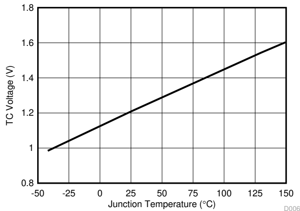
FIG 6-9. TC Voltage versus Temperature
