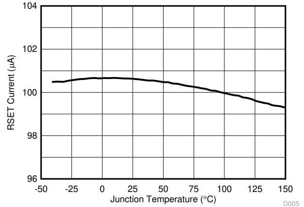
FIG 6-8. RSET Current versus Temperature
