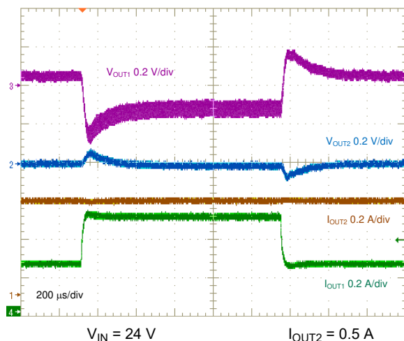
V_{IN} = 24\text{ V} I_{OUT2} = 0.5\text{ A} 図 8-25. Positive Output Load Transient, 0.25 A to 0.5 A
