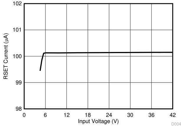
FIG 6-7. RSET Current versus Input Voltage
