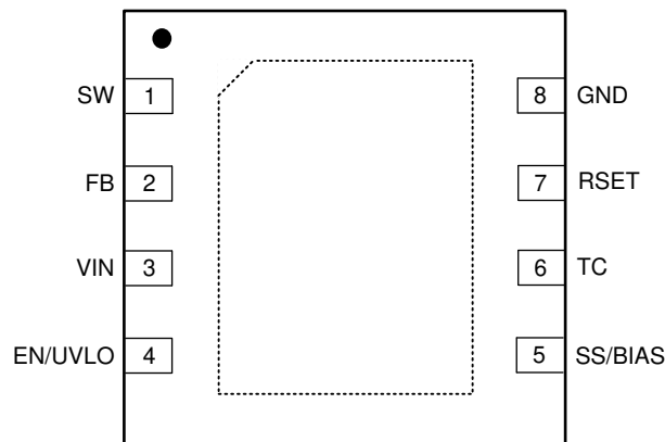
FIG 5-1. 8-Pin WSON NGU Package With Wettable Flanks (Top View)
