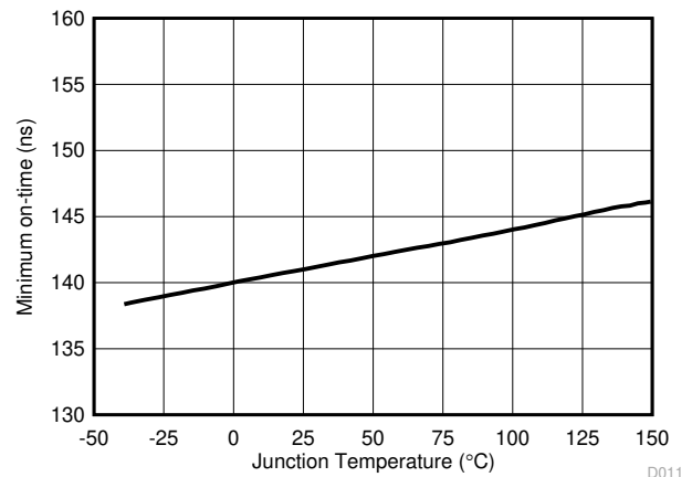
FIG 6-12. Minimum Switch On-Time versus Temperature
