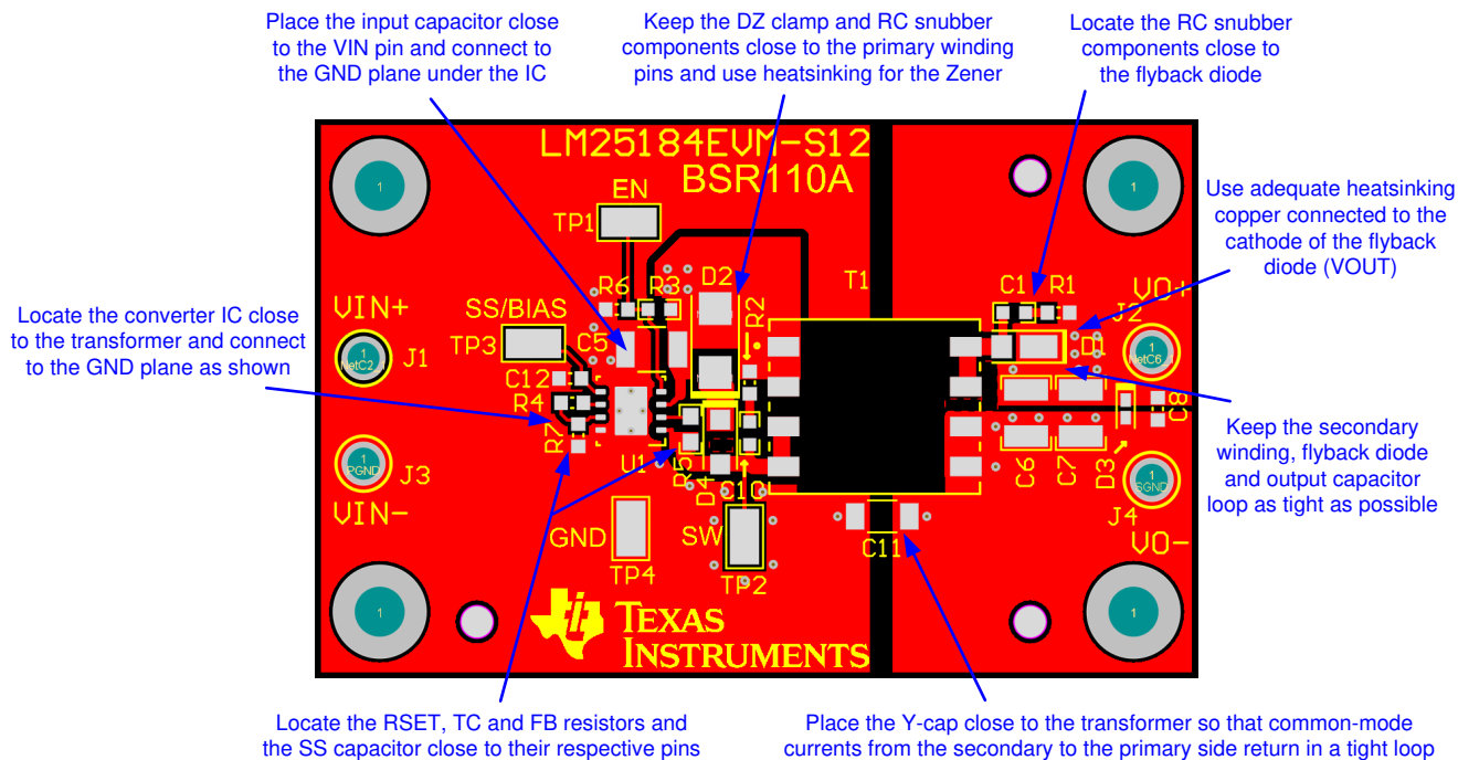
FIG 10-1. Single-Output PCB Layout Example
