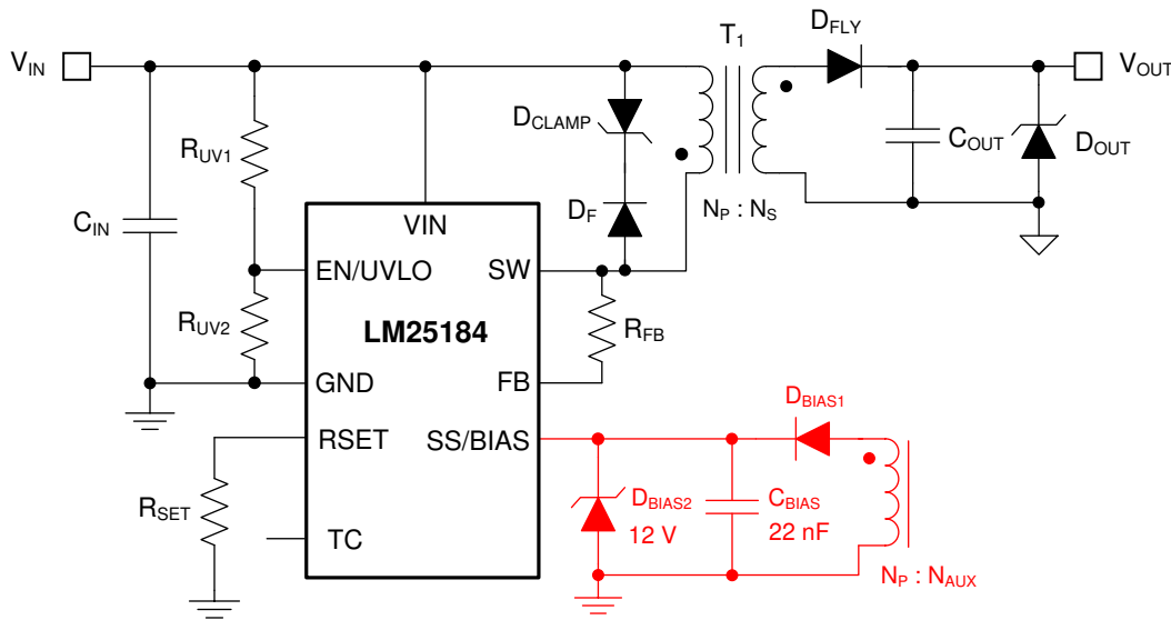
FIG 7-4. External Bias Supply Using Transformer Auxiliary Winding
