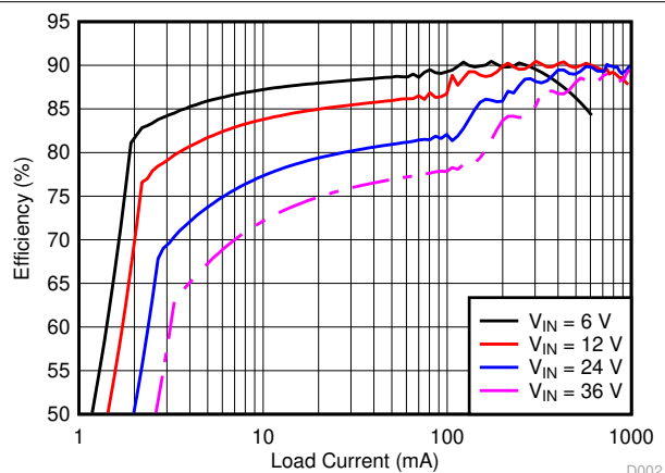
图 8-3. Efficiency (Log Scale)
