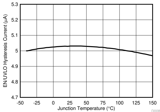
FIG 6-11. EN/UVLO Hysteresis Current versus Temperature
