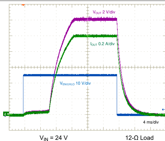
图 8-7. Enable ON and OFF Characteristic
