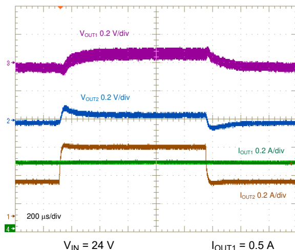
V_{IN} = 24\text{ V} I_{OUT1} = 0.5\text{ A} 図 8-26. Negative Output Load Transient, 0.25 A to 0.5 A
