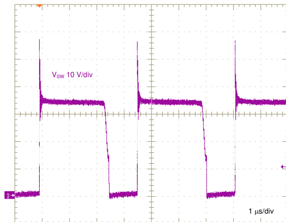
V_{IN} = 24\text{ V} I_{OUT1} = I_{OUT2} = 0.5\text{ A} 図 8-24. Switch Voltage, Full Load
