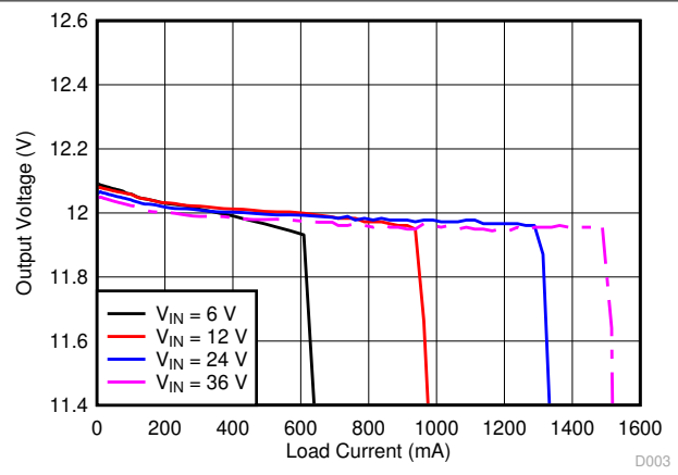
6-2. Output Voltage versus Load
