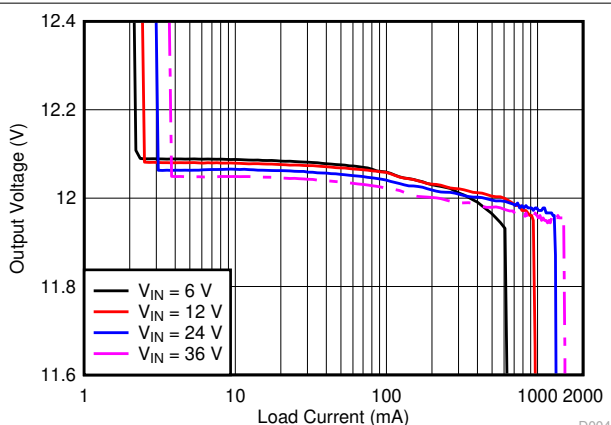
8-5. Load Regulation (Log Scale)
