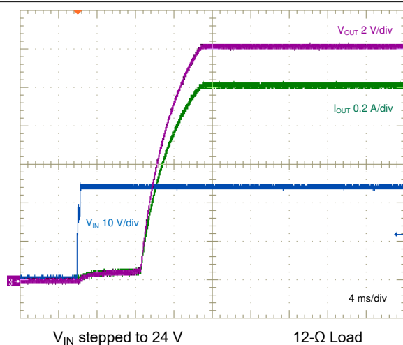
8-6. Start-up Characteristic
