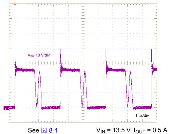
6-4. Switching Waveform in DCM
