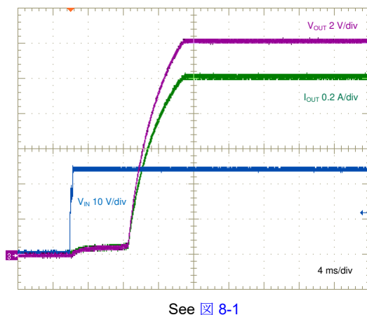
6-5. Start-up Characteristic
