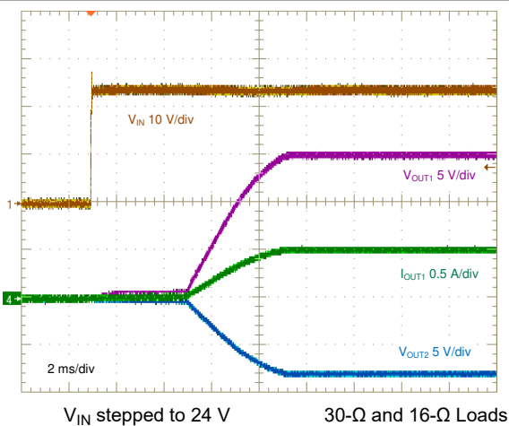
8-21. Start-Up Characteristic
