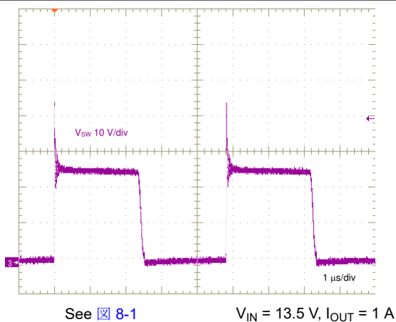
6-3. Switching Waveform in BCM
