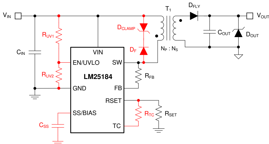
FIG 7-1. LM25184 Flyback Converter Schematic (Optional Components in Red)
