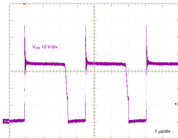
8-24. Switch Voltage, Full Load
