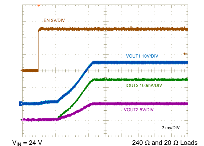
FIG 48. ENABLE ON Characteristic
