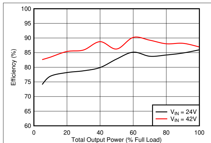
FIG 46. Efficiency
