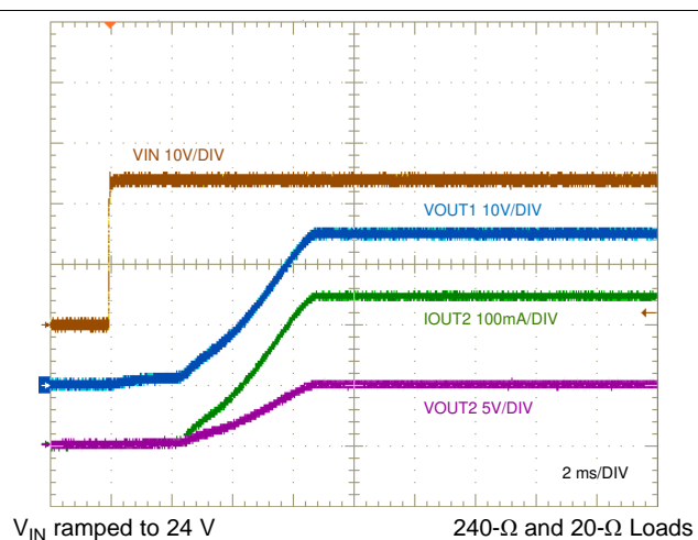
FIG 47. Start-Up Characteristic
