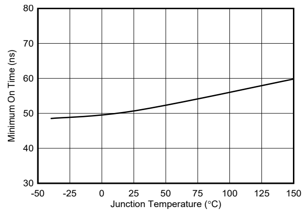
FIG 7-20. Minimum On Time (HO) vs Temperature
