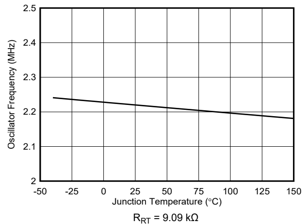
FIG 7-22. Switching Frequency vs Temperature
