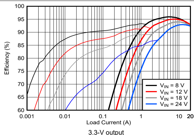
図 9-30. Efficiency vs I_{OUT} , Log Scale
