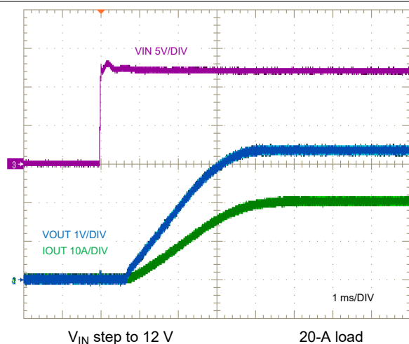
図 9-31. V_{IN} Start-Up Characteristic
