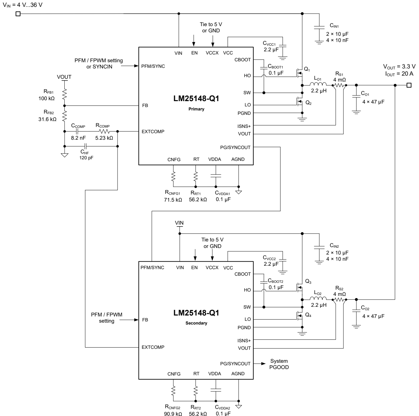
9-28. Application Circuit 3 With Two LM25148-Q1 Buck Regulators Switching at 400 kHz
