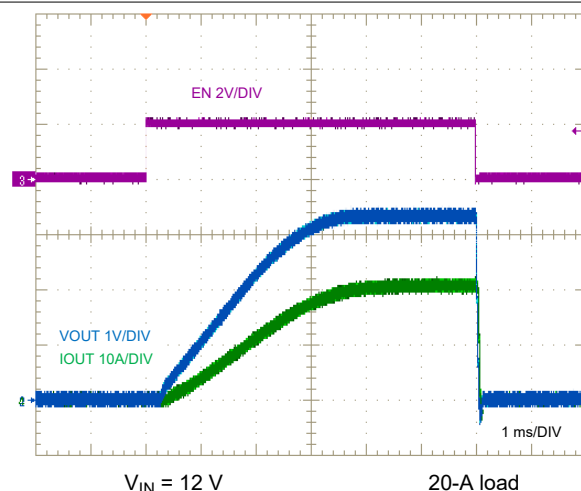
図 9-32. ENABLE ON and OFF Characteristic
