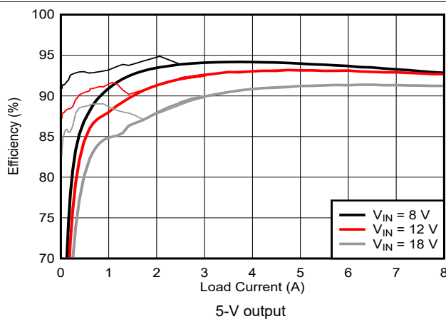
図 9-5. Efficiency vs I_{OUT}
