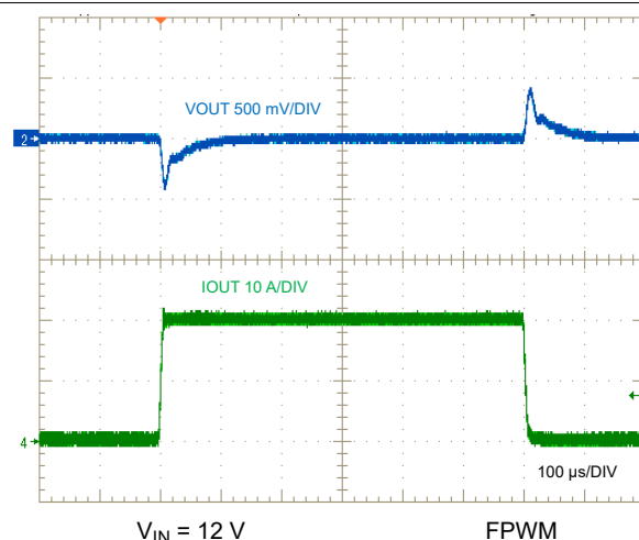
図 9-34. Load Transient, 0 A to 20 A
