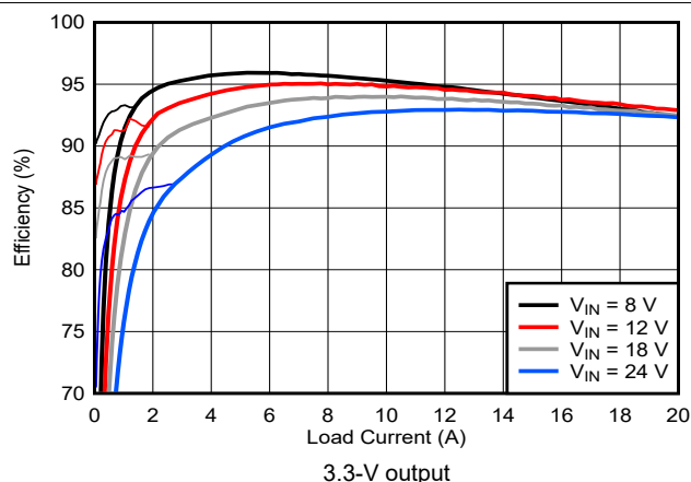
図 9-29. Efficiency vs I_{OUT}
