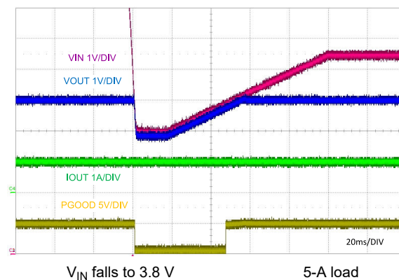
図 9-10. Cold-Crank Response to V_{IN} = 3.8 V
