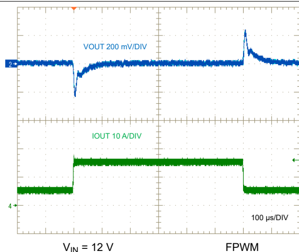
図 9-33. Load Transient, 5 A to 15 A
