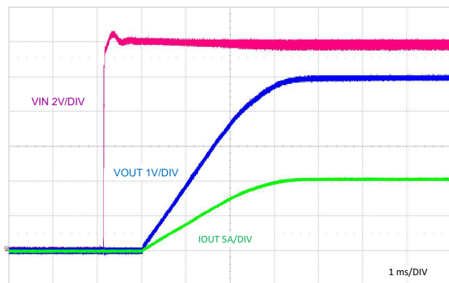
9-24. Start-Up Characteristic
