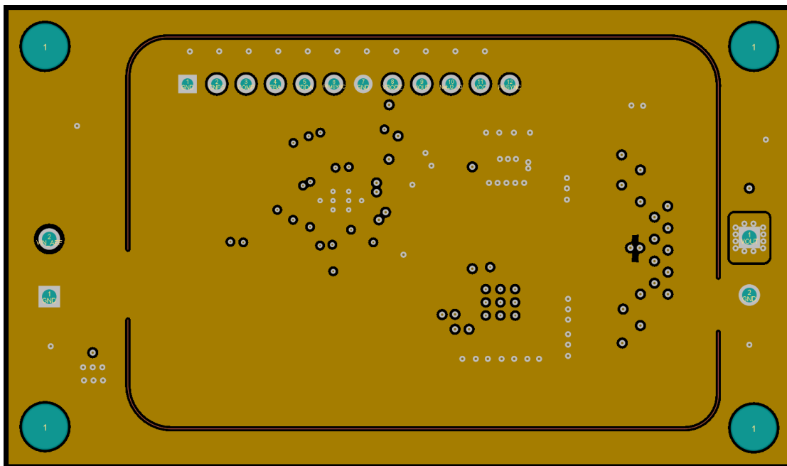
11-3. Layer 2 Full Ground Plane Directly Under the Power Components
