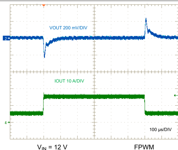
9-33. Load Transient, 5 A to 15 A
