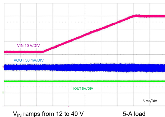
9-22. Line Transient Response to V_{IN} = 40 V
