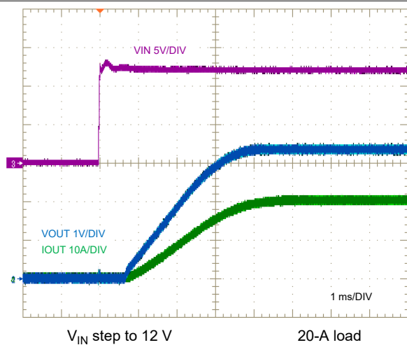
9-31. V_{IN} Start-Up Characteristic
