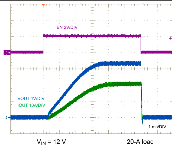
9-32. ENABLE ON and OFF Characteristic
