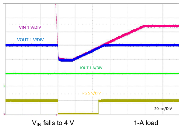
9-23. Cold-Crank Response to V_{IN} = 4\text{ V}
