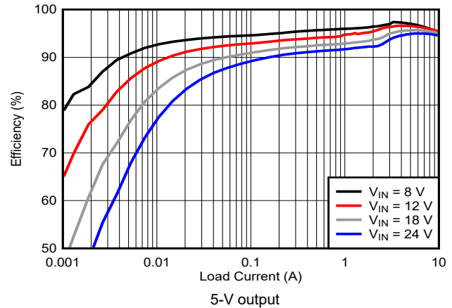
9-19. Efficiency vs I_{OUT} , Log Scale
