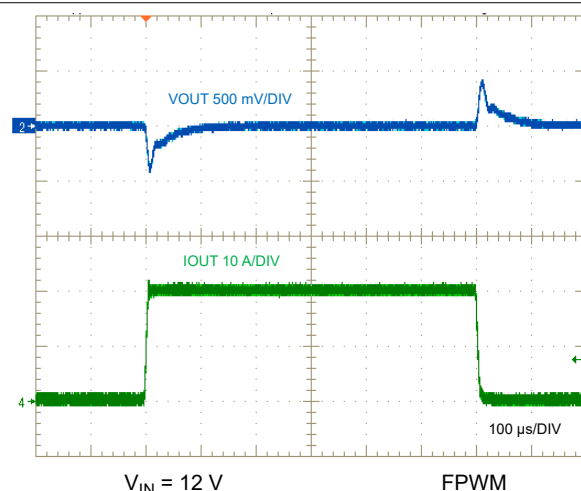
9-34. Load Transient, 0 A to 20 A
