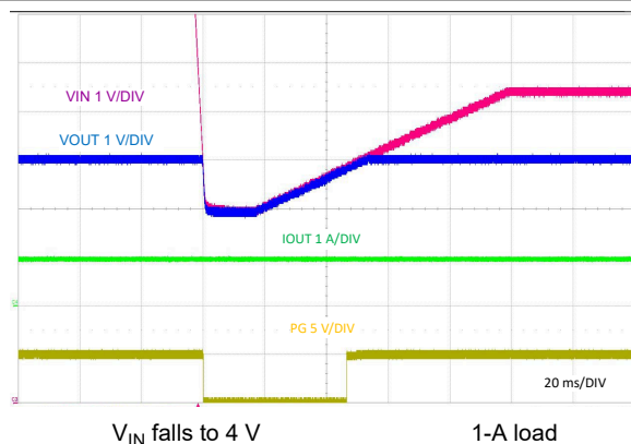
9-23. Cold-Crank Response to V_{IN} = 4 V
