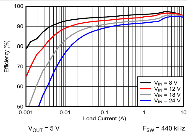
7-2. Efficiency vs. Load, Log Scale
