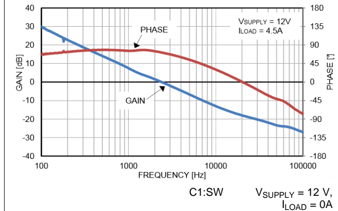
Figure 46. Loop Response
