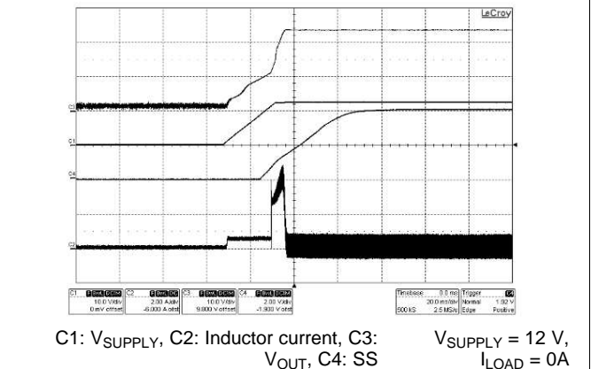
Figure 47. Start-Up
