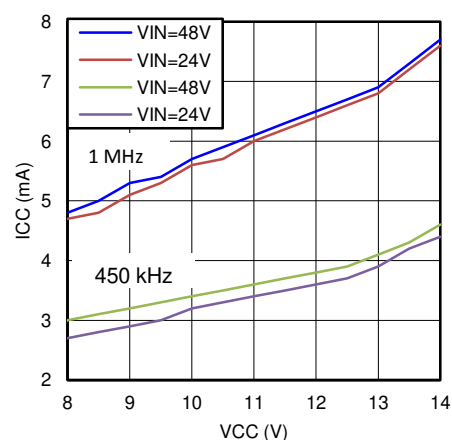
Figure 6-4. I_{CC} versus External V_{CC}
