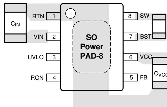
❏ 10-1. Placement of Bypass Capacitors
