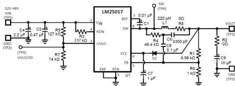
8-1. Final Schematic for 12.5-V to 48-V Input, and 10-V, 650-mA Output Buck Converter
