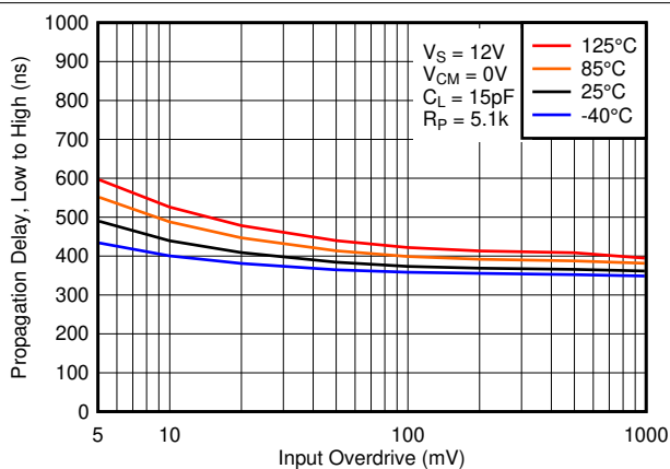
FIG 6-28. Low to High Propagation Delay vs. Input Overdrive Voltage, 12V
