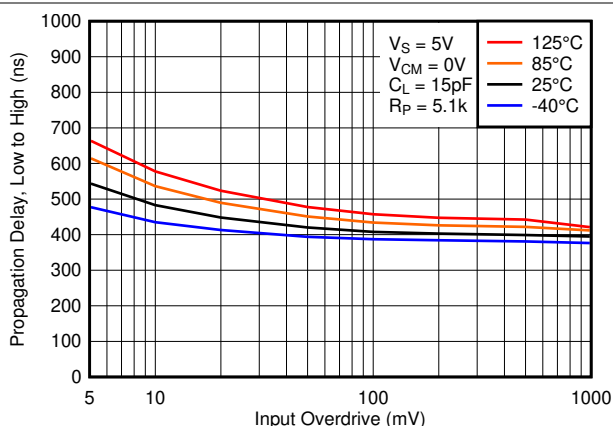
FIG 6-26. Low to High Propagation Delay vs. Input Overdrive Voltage, 5V
