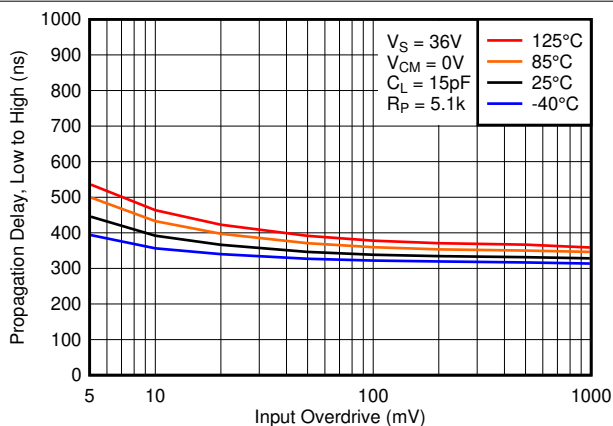
FIG 6-30. Low to High Propagation Delay vs. Input Overdrive Voltage, 36V
