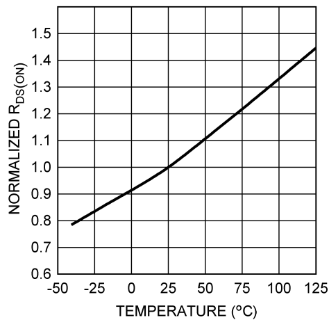
FIG 6-4. Normalized R_{DS(ON)} vs Temperature
