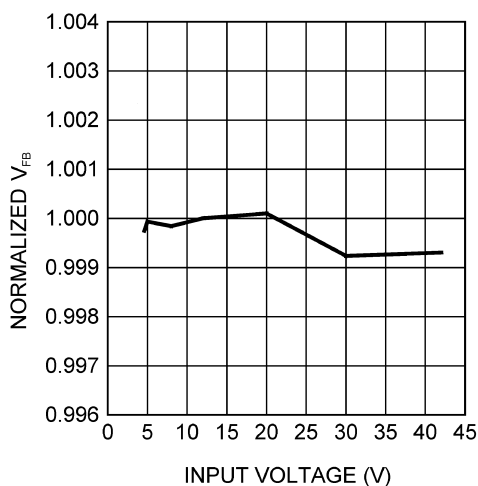
6-9. Normalized Feedback Voltage vs Input Voltage
