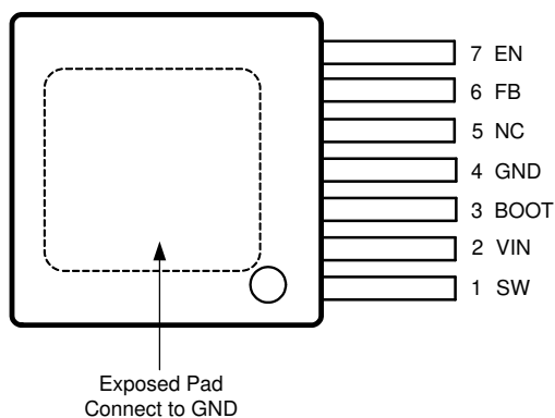
✎ 5-1. 7-Pin PFM Package (Top View)
