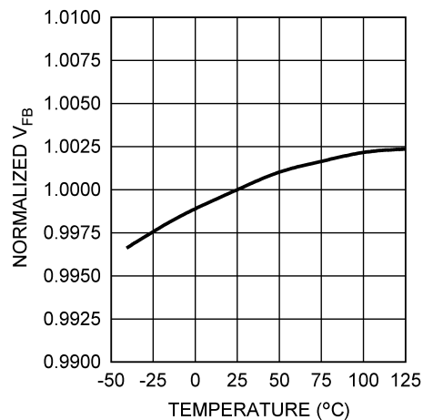
6-8. Normalized Feedback Voltage vs Temperature
