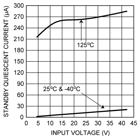
6-7. Standby Quiescent Current vs Input Voltage
