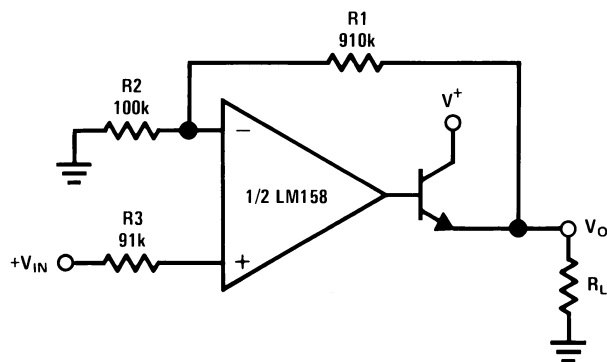
8-4. Power Amplifier
