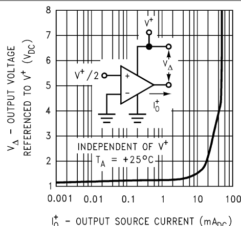
6-10. Output Characteristics Current Sourcing
