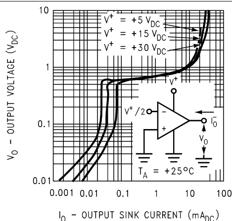
6-11. Output Characteristics Current Sinking
