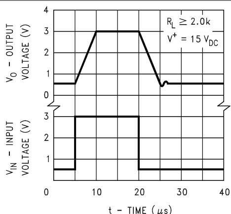
6-7. Voltage Follower Pulse Response
