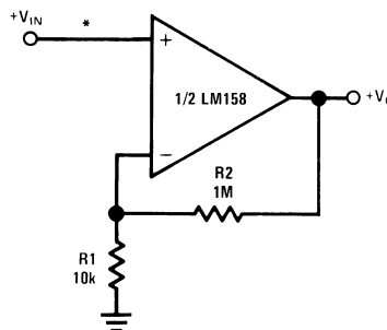
✕ 8-1. Non-Inverting DC Gain (0-V Output)
