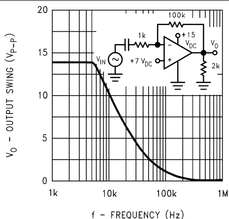
6-9. Large Signal Frequency Response
