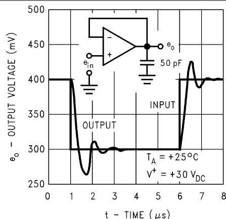
6-8. Voltage Follower Pulse Response (Small Signal)
