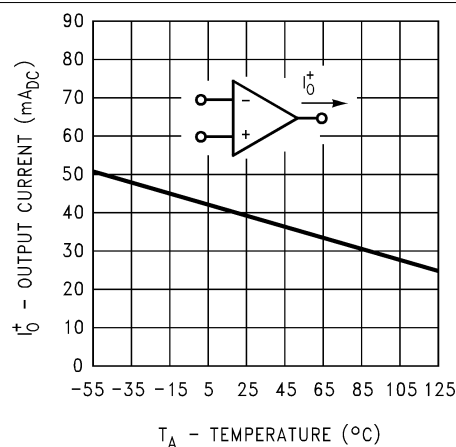
6-12. Current Limiting
