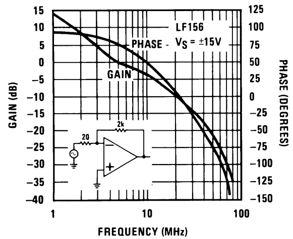
Figure 26. Bode Plot
