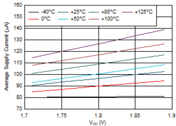
FIG 6-6. Supply Current vs. V_{DD} . Sensor R_P = 720\ \Omega , Scan Rate = 40 SPS, Sensor Frequency = 20 MHz.
