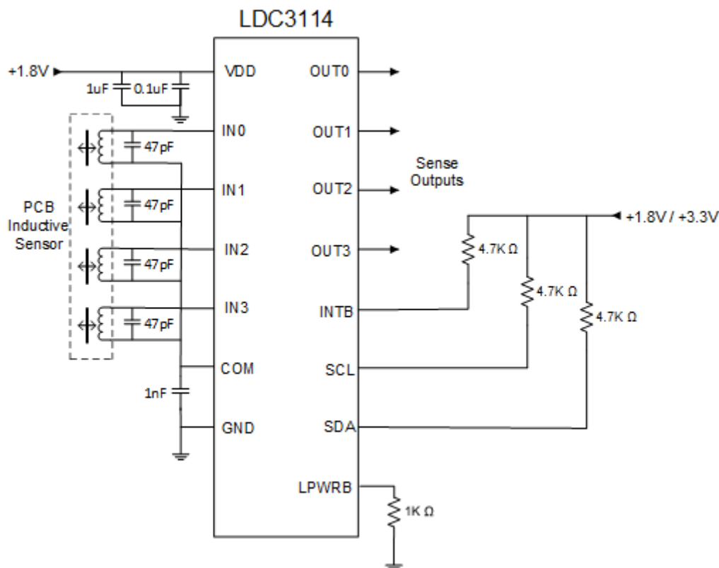
FIG 8-15. Application Schematic
