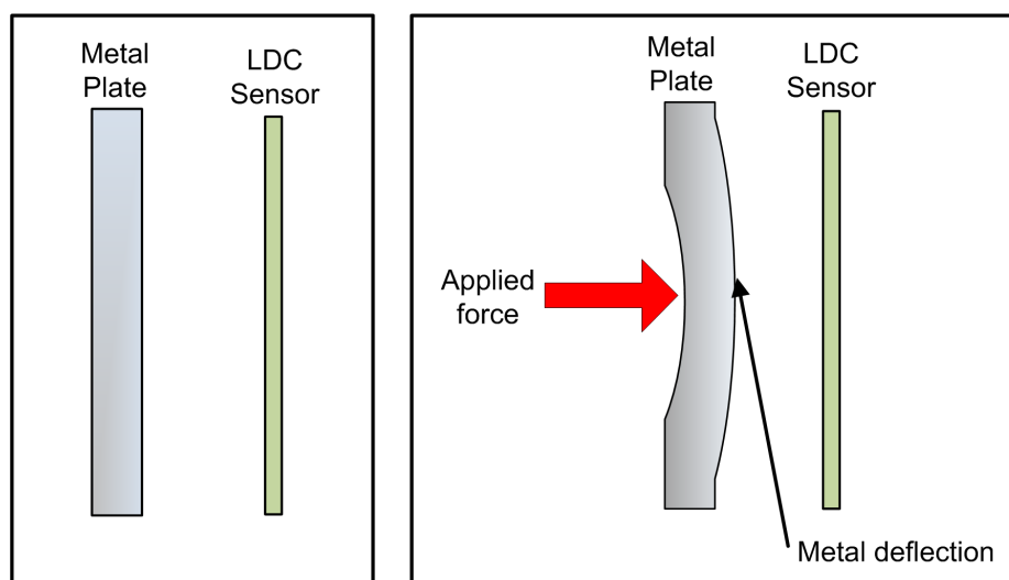
Figure 8-1. Metal Deflection
