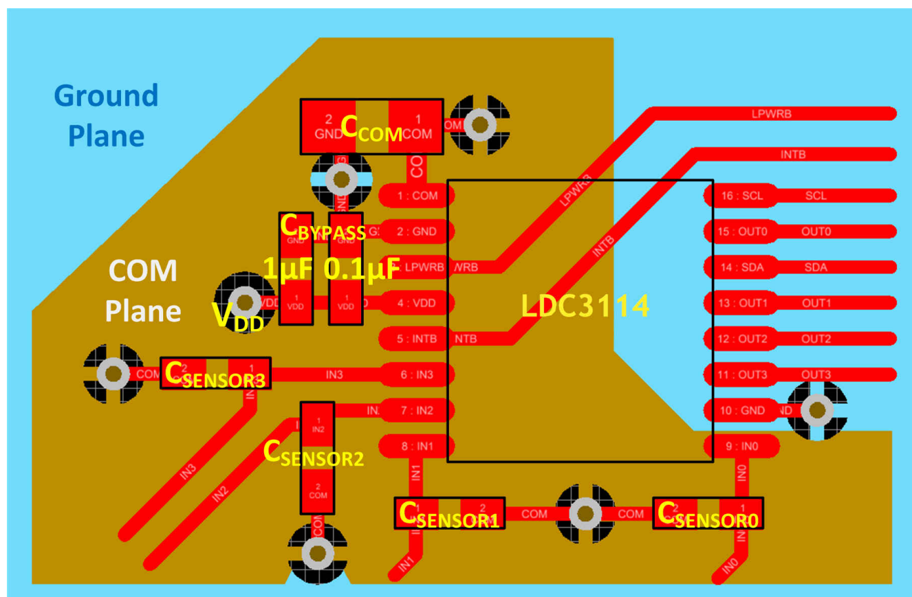
FIG 10-1. Layout of LDC3114 (TSSOP-16) With Decoupling Capacitors and Sensor Capacitors
