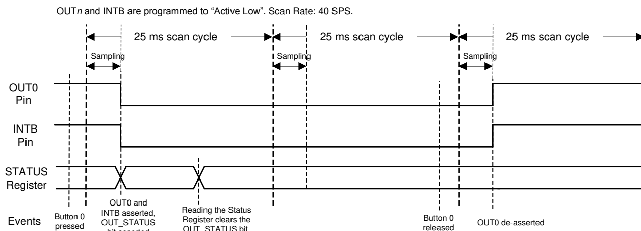
8-13. Timing Diagram of a Single Button Press
