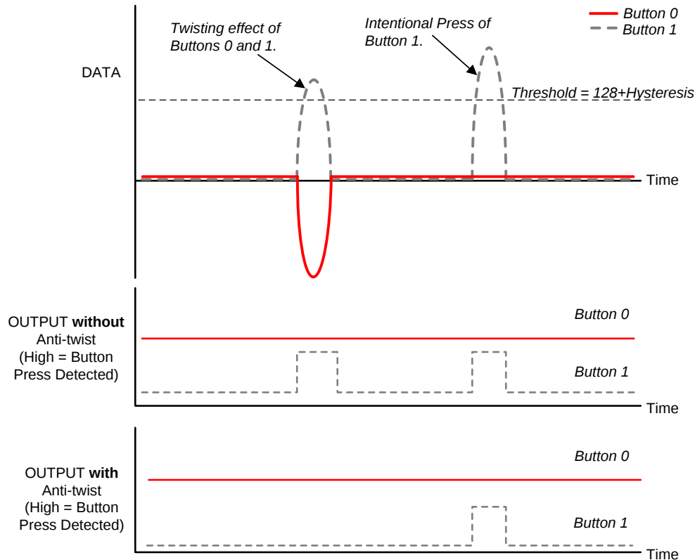
FIG 28. Illustration of the Anti-Twist Feature
