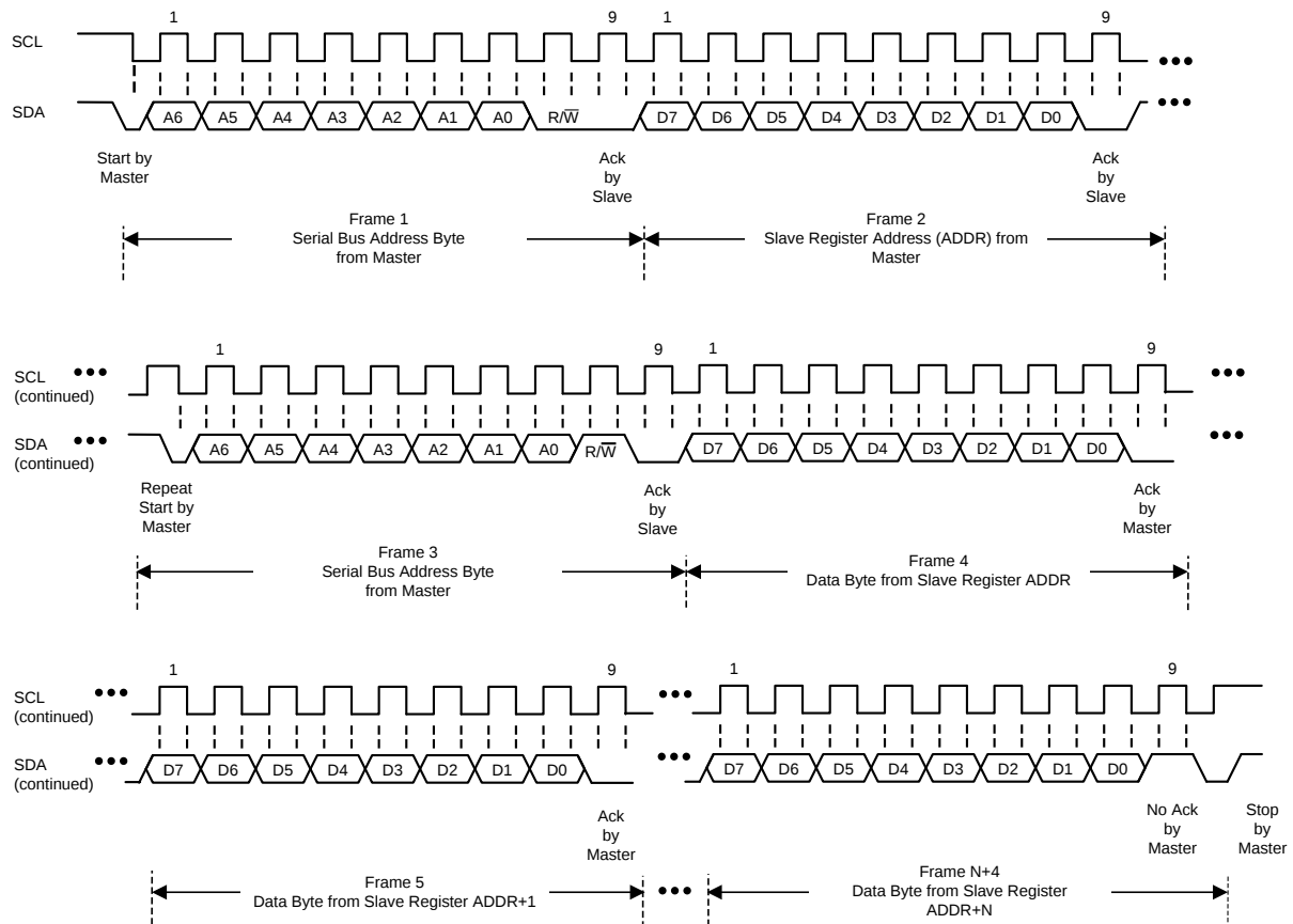
FIG 16. I²C Sequence of Reading Consecutive Registers
