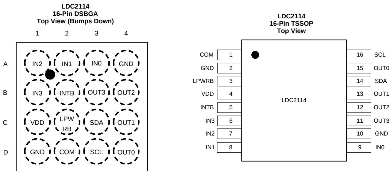
Pin Functions - LDC2114
