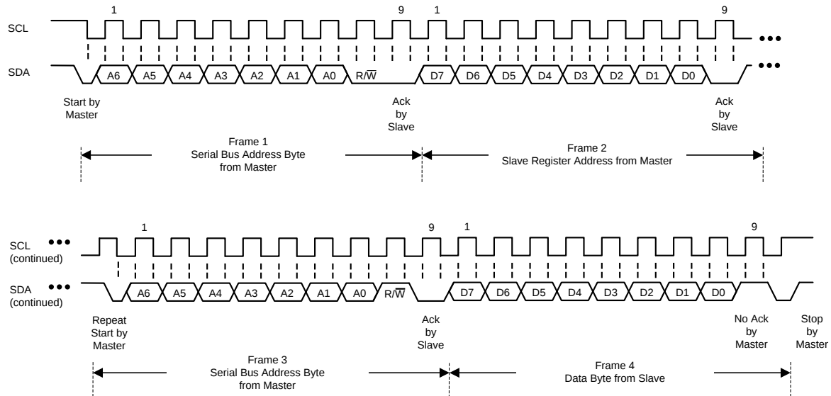
FIG 15. I²C Sequence of Reading a Single Register
