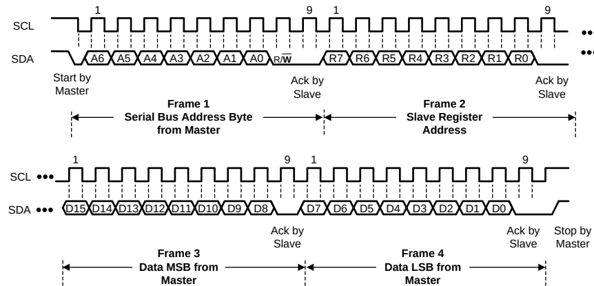
Figure 14. I2C Write Register Sequence
