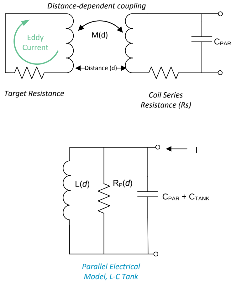
Figure 50. Electrical Model of the L-C Tank Sensor
