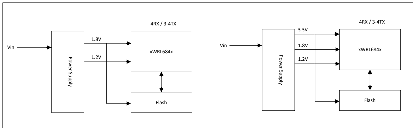
图 7-2. I/O Topologies (Left: 1.8V I/O Topology, Right: 3.3V I/O Topology)
