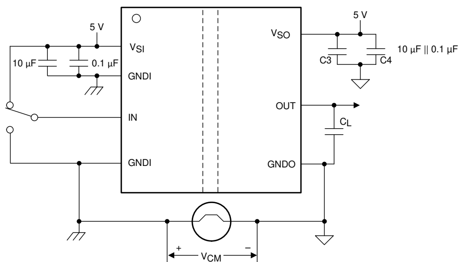
⊗ 24. Switching Characteristics Test Circuit and Voltage Waveforms
