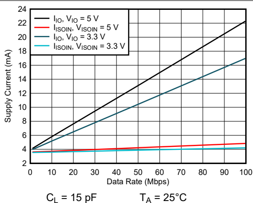
7-19. ISOW7744 Channel Supply Currents vs Data Rate For C_L = 15 \text{ pF}
