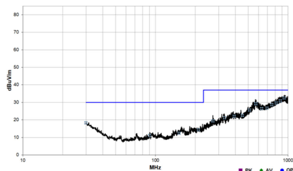
FIG 10-3. ISOW7741 Radiated Emissions versus CISPR32B line (Blue)
