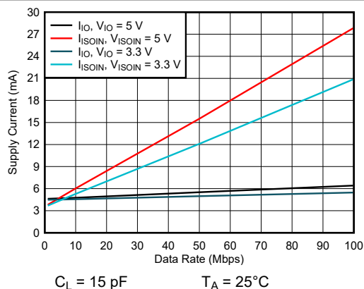
7-11. ISOW7740 Channel Supply Currents vs Data Rate For C L = 15 pF
