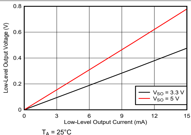
7-24. Low-Level Output Voltage vs Low-Level Output Current
