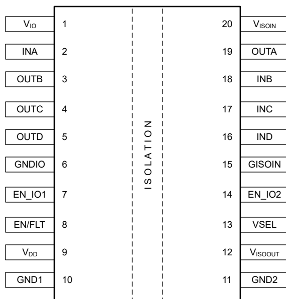
FIG 6-4. ISOW7743 DFM Package 20-Pin SOIC-WB Top View
