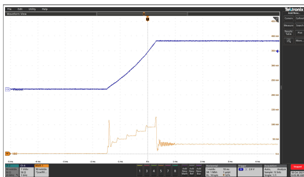
7-26. Soft Start at 10-mA Load For V_{ISOOUT} = 3.3 V
