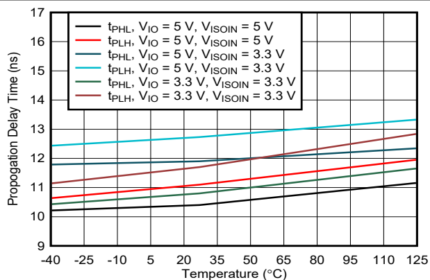
7-22. Propagation Delay Time vs Free-Air Temperature
