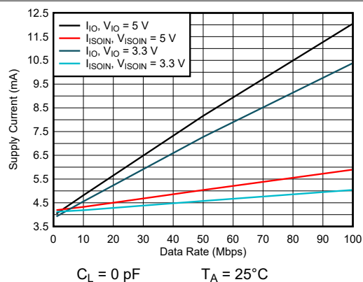
7-20. ISOW7744 Channel Supply Currents vs Data Rate For C_L = 0 \text{ pF}
