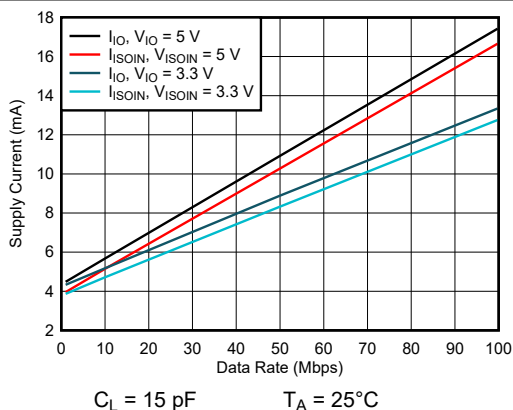
7-15. ISOW7742 Channel Supply Currents vs Data Rate For C_L = 15 \text{ pF}
