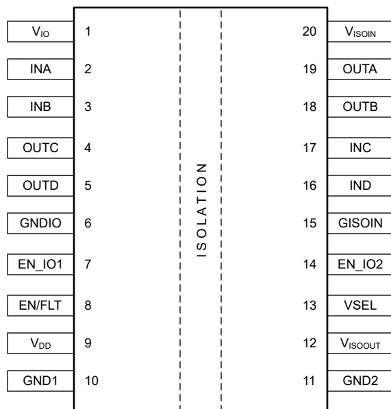
6-3. ISOW7742 DFM Package 20-Pin SOIC-WB Top View
