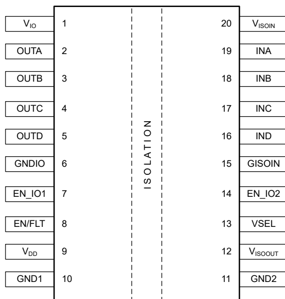
FIG 6-5. ISOW7744 DFM Package 20-Pin SOIC-WB Top View
