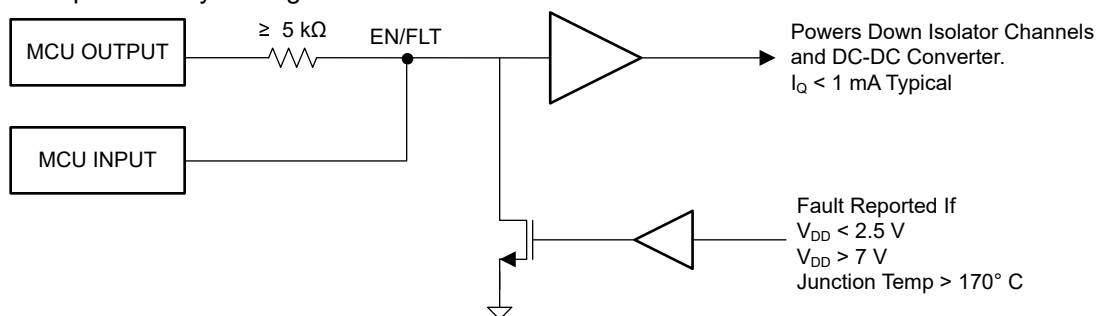
9-4. EN/FLT Fault Pin Diagram
