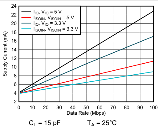
7-17. ISOW7743 Channel Supply Currents vs Data Rate For C_L = 15 \text{ pF}
