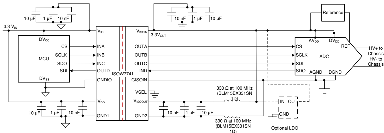
10-1. Isolated Power and SPI for ADC Sensing Application with ISOW7741
