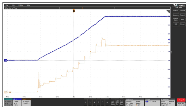
7-29. Soft Start at 10-mA Load For V_{ISOOUT} = 5\text{ V}
