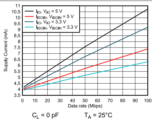
7-18. ISOW7743 Channel Supply Currents vs Data Rate For C_L = 0 \text{ pF}
