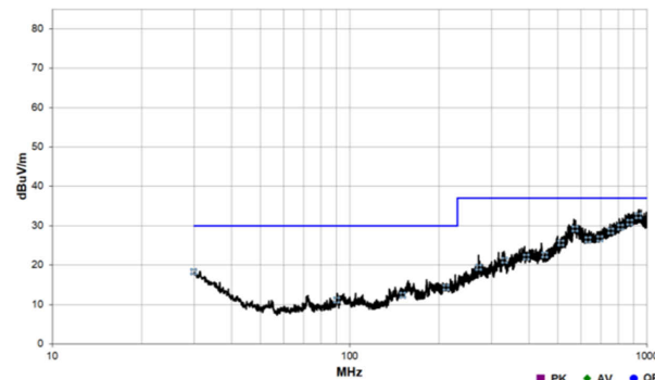
FIG 10-3. ISOW7741 Radiated Emissions versus CISPR32B line (Blue)
