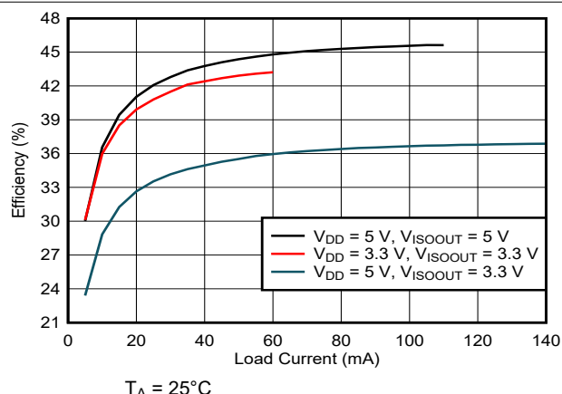
7-6. Efficiency vs Load Current ( I_{ISOOUT} )
