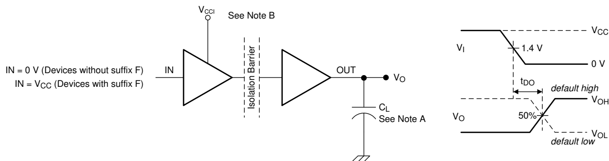
8-2. Enable/Disable Propagation Delay Time Test Circuit and Waveform
