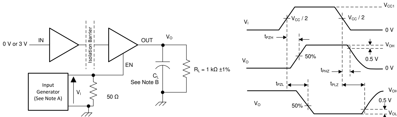
8-1. Switching Characteristics Test Circuit and Voltage Waveforms
