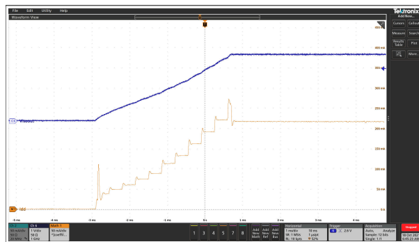
7-18. Soft Start at 10-mA Load For V_{ISOOUT} = 3.3\text{ V}
