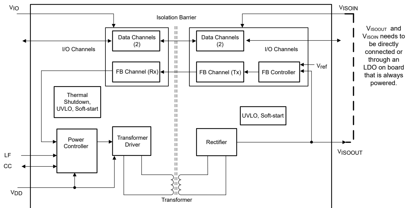
9-1. Block Diagram
