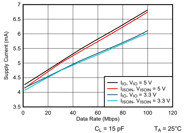
7-12. ISOW7721 Channel Supply Currents vs Data Rate For C L = 0 pF
