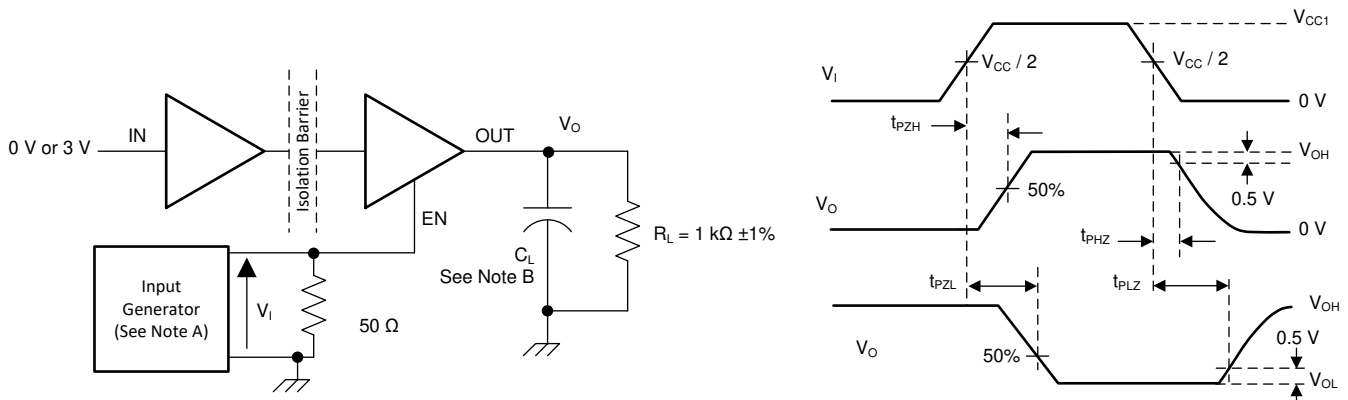
8-1. Switching Characteristics Test Circuit and Voltage Waveforms
