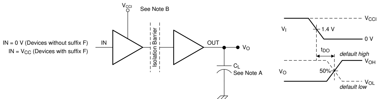
8-2. Enable/Disable Propagation Delay Time Test Circuit and Waveform
