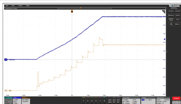
7-21. Soft Start at 10-mA Load For V_{ISOOUT} = 5\text{ V}
