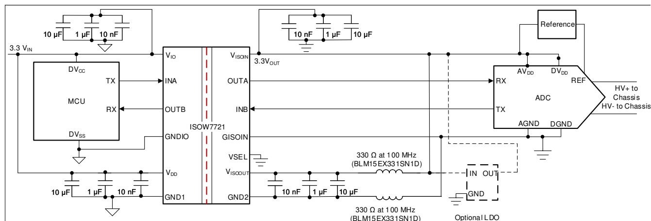
10-1. Isolated Power and UART for ADC Sensing Application with ISOW7721
