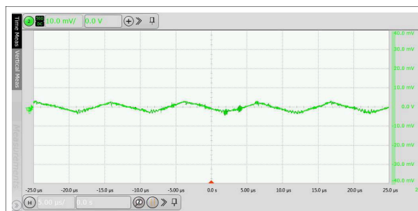
7-24. V_{ISOOUT} Ripple Voltage at 3.3 V with 10 \mu\text{F} Capacitor and 60 mA load
