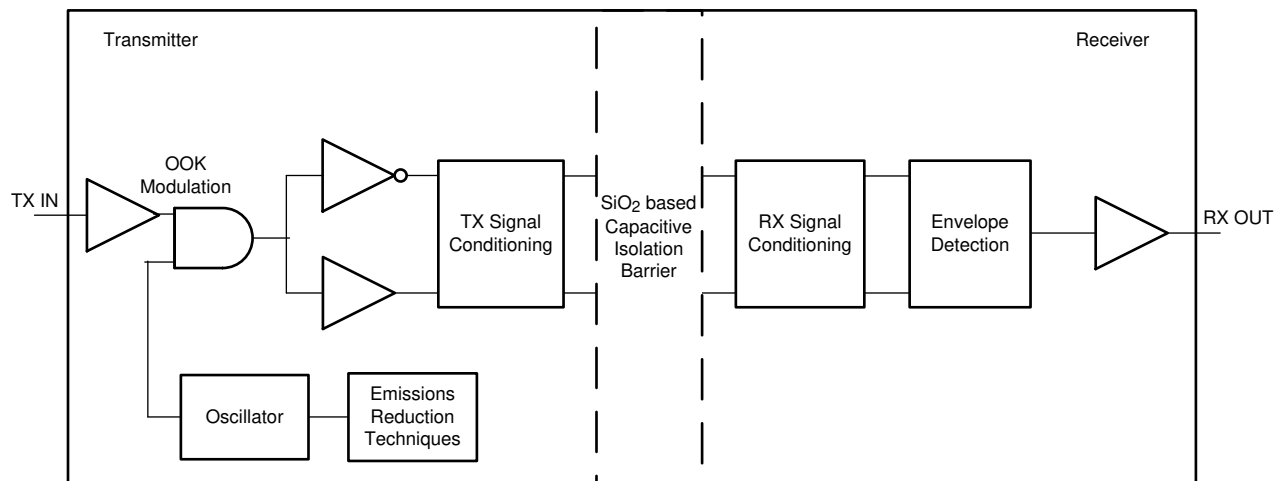
9-2. Conceptual Block Diagram of a Capacitive Data Channel
