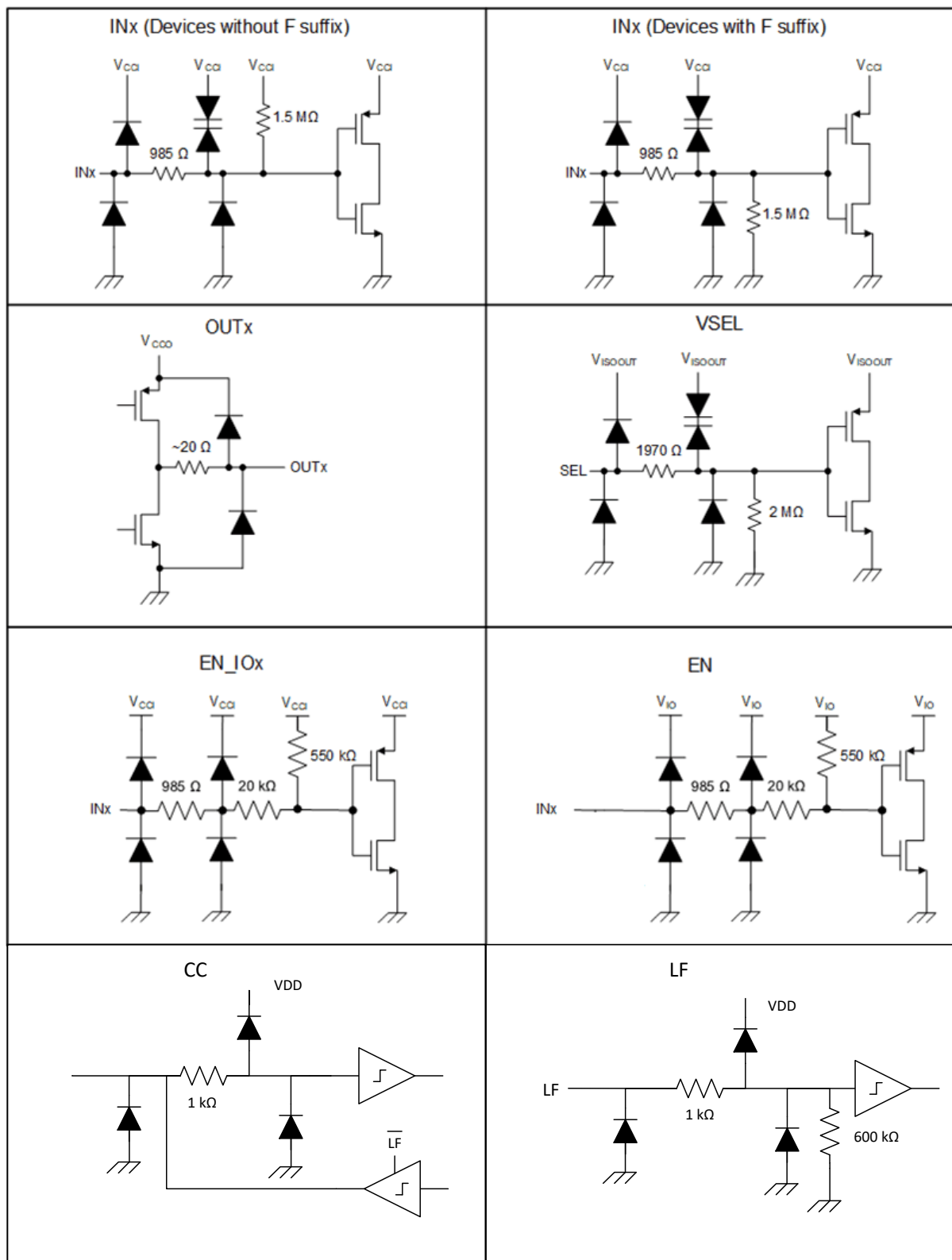
9-5. Device I/O Schematics
