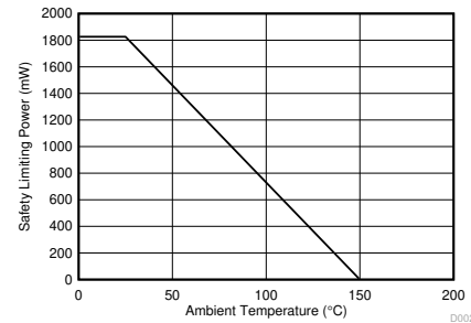
8-2. Thermal Derating Curve for Limiting Power per VDE
