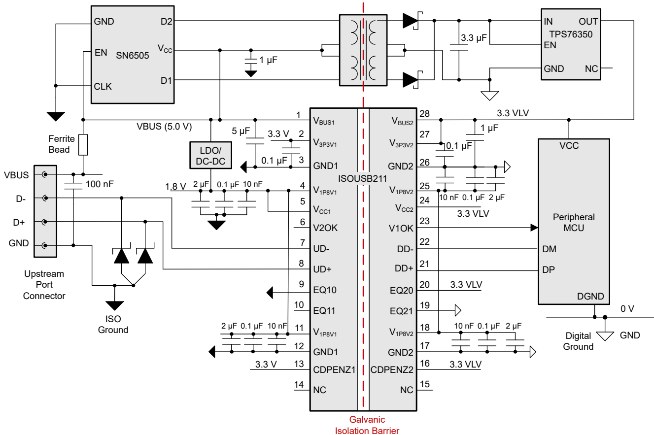
図 8-3. Isolated Bus-Powered Peripheral using ISOUSB211-Q1
