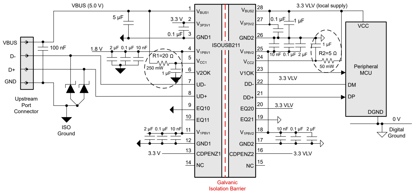
图 8-8. Using ISOUSB211-Q1 with Resistors in series with V CCx pins
