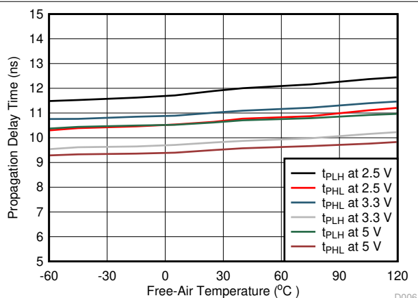
5-8. Propagation Delay Time vs Free-Air Temperature
