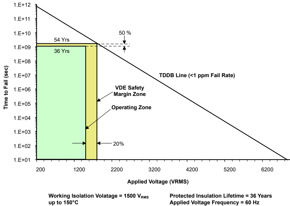
図 8-7. Insulation Lifetime Projection Data
