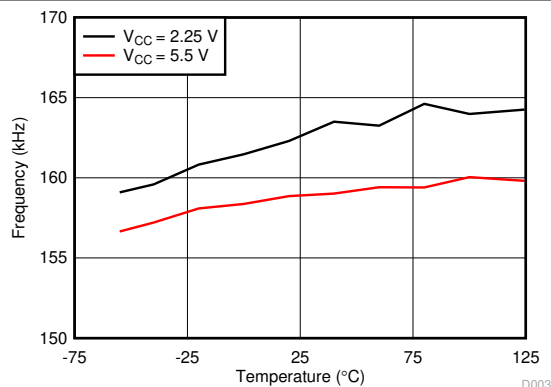
図 5-15. ISO774xTA-Q1 Frequency vs. Free-Air Temperature
