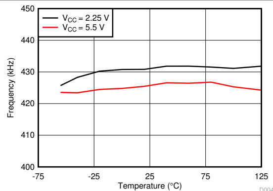
図 5-16. ISO774xTB-Q1 Frequency vs. Free-Air Temperature
