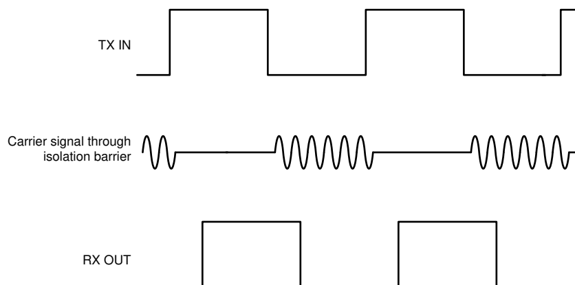
7-2. On-Off Keying (OOK) Based Modulation Scheme
