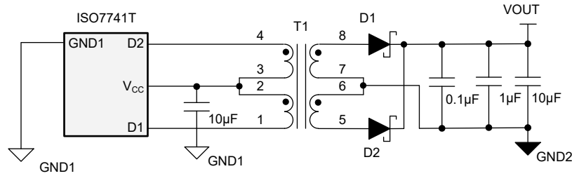
図 8-5. Unregulated Output for Low-Current Loads With Wide Supply Range
