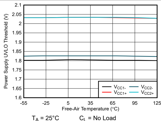
5-10. Power Supply Undervoltage Threshold vs. Free-Air Temperature
