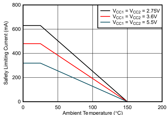
図 5-1. Thermal Derating Curve for Safety Limiting Current for DW-16 Package
