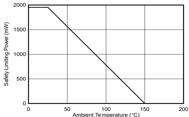
図 5-2. Thermal Derating Curve for Safety Limiting Power for DW-16 Package
