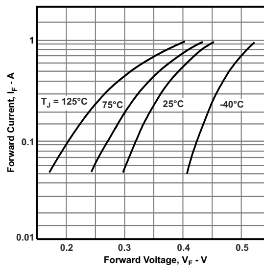
図 8-3. Diode Forward Characteristics MBR0530
