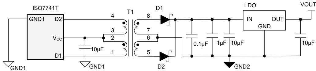
図 8-6. Regulated Output for Stable Supplies and High Current Loads
