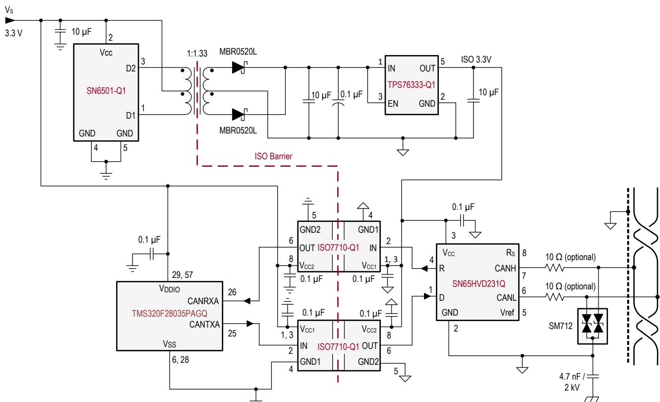
図 25-1. Isolated CAN Interface
