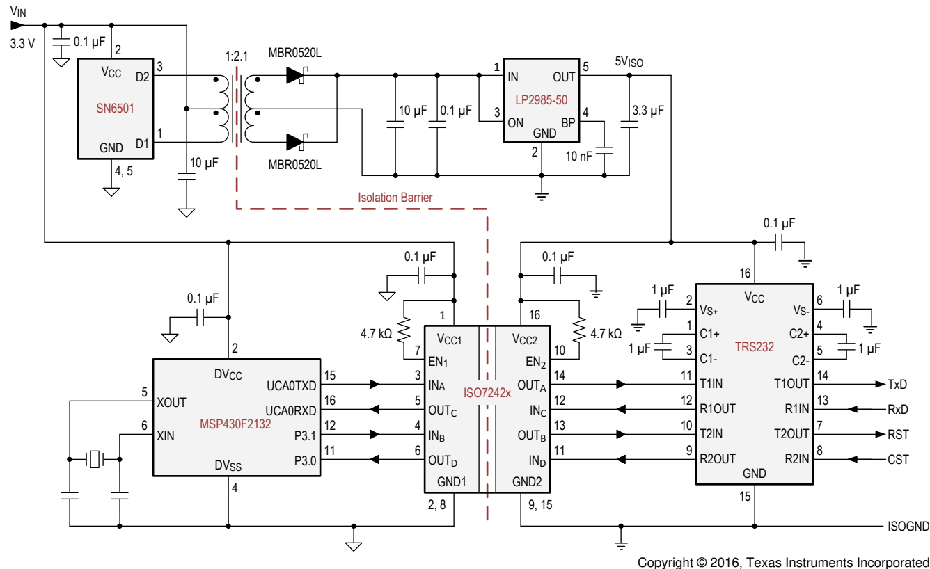
8-9. Isolated RS-232 Interface
