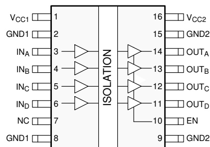
図 4-2. ISO7240C DW Package 16-Pin SOIC Top View
