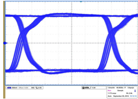
図 8-7. ISO7242M Eye Diagram at 150 Mbps, 3.3 V and 25°C
