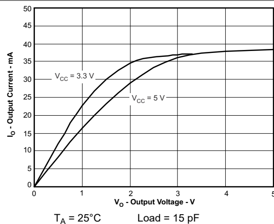
図 5-10. Low-Level Output Current vs Low-Level Output Voltage
