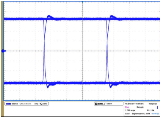
図 8-6. ISO7242M Eye Diagram at 25 Mbps, 3.3 V and 25°C
