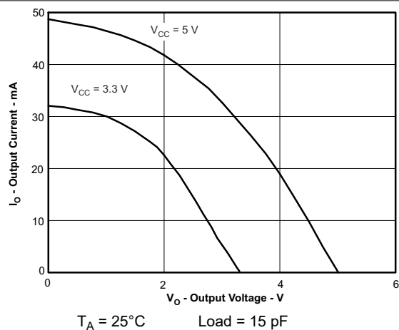
図 5-9. High-Level Output Current vs High-Level Output Voltage
