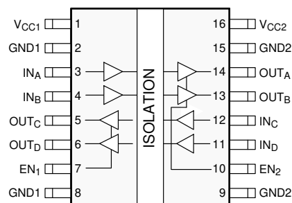
图 4-4. ISO7242C DW Package 16-Pin SOIC Top View
