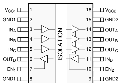
图 4-3. ISO7241C DW Package 16-Pin SOIC Top View
