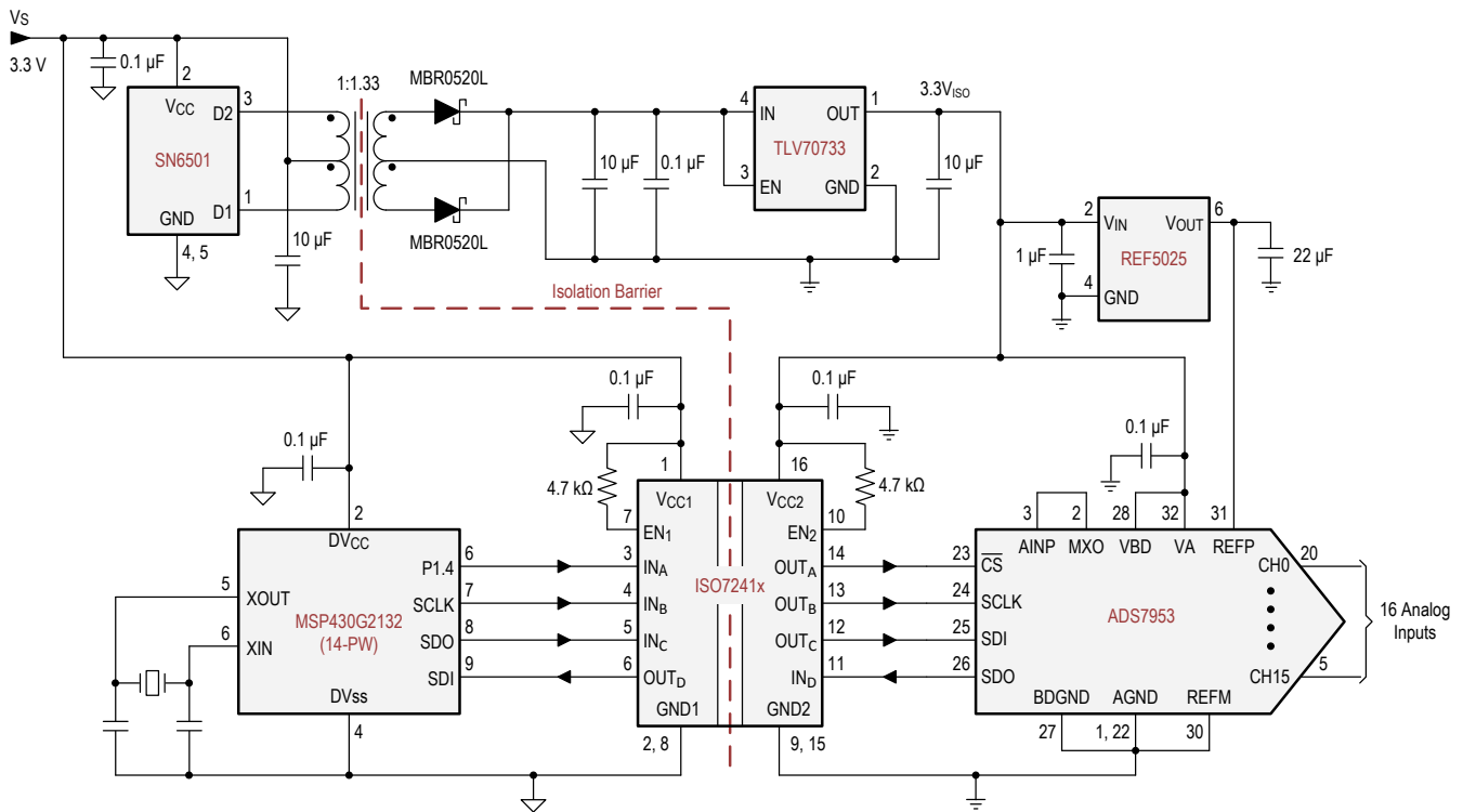
図 8-8. Isolated SPI for an Analog Input Module With 16 Inputs
