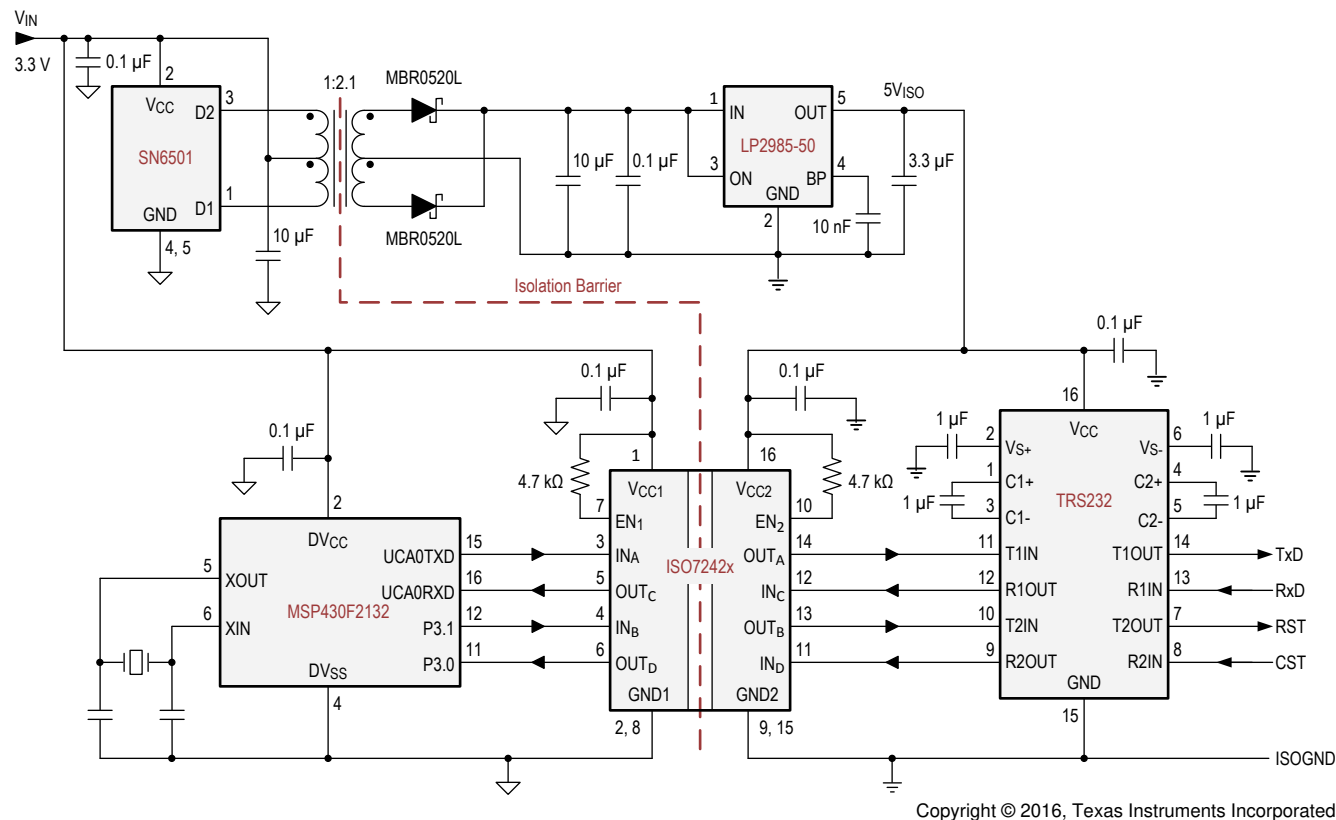
図 8-9. Isolated RS-232 Interface
