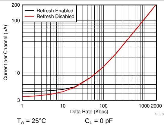
FIG 5. ISO7041 Supply Current vs Data Rate at 3.3 V (With No Load)
