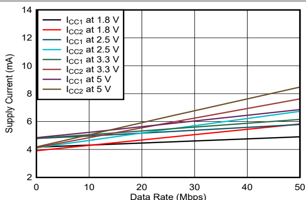
FIG 6-4. ISO6760-Q1 Supply Current vs Data Rate (With No Load)
