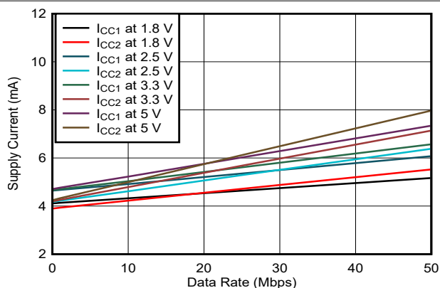
FIG 6-6. ISO6761-Q1 Supply Current vs Data Rate (With No Load)
