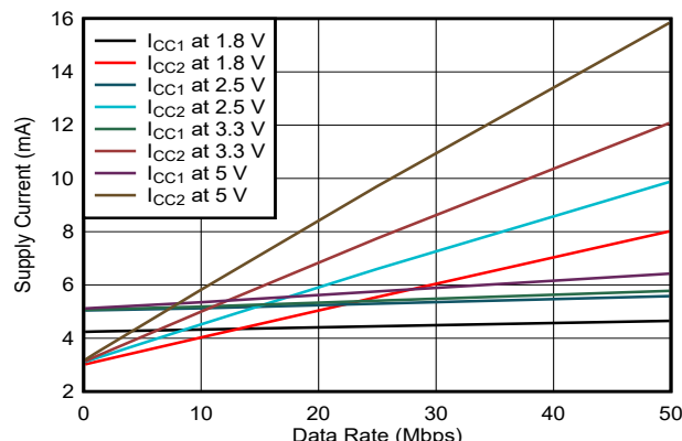
FIG 6-3. ISO6760-Q1 Supply Current vs Data Rate (With 15-pF Load)
