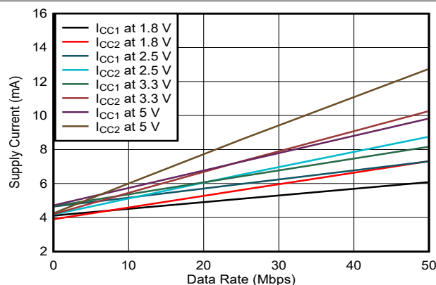
FIG 6-5. ISO6761-Q1 Supply Current vs Data Rate (With 15-pF Load)
