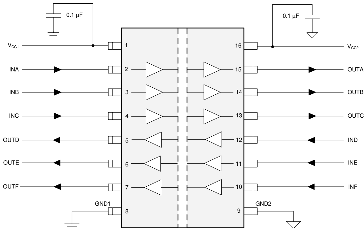
图 9-2. Typical ISO676x-Q1 Circuit Hook-up
