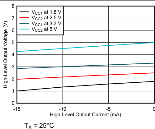
6-11. High-Level Output Voltage vs High-level Output Current
