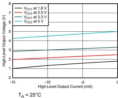
FIG 6-11. High-Level Output Voltage vs High-level Output Current
