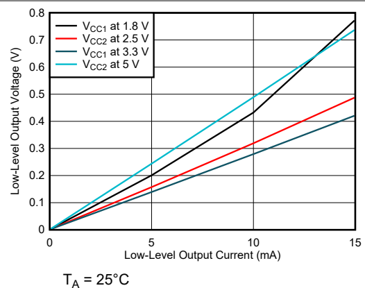
FIG 6-14. Low-Level Output Voltage vs Low-Level Output Current
