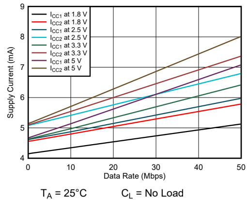
FIG 6-10. ISO6763 Supply Current vs Data Rate (With No Load)
